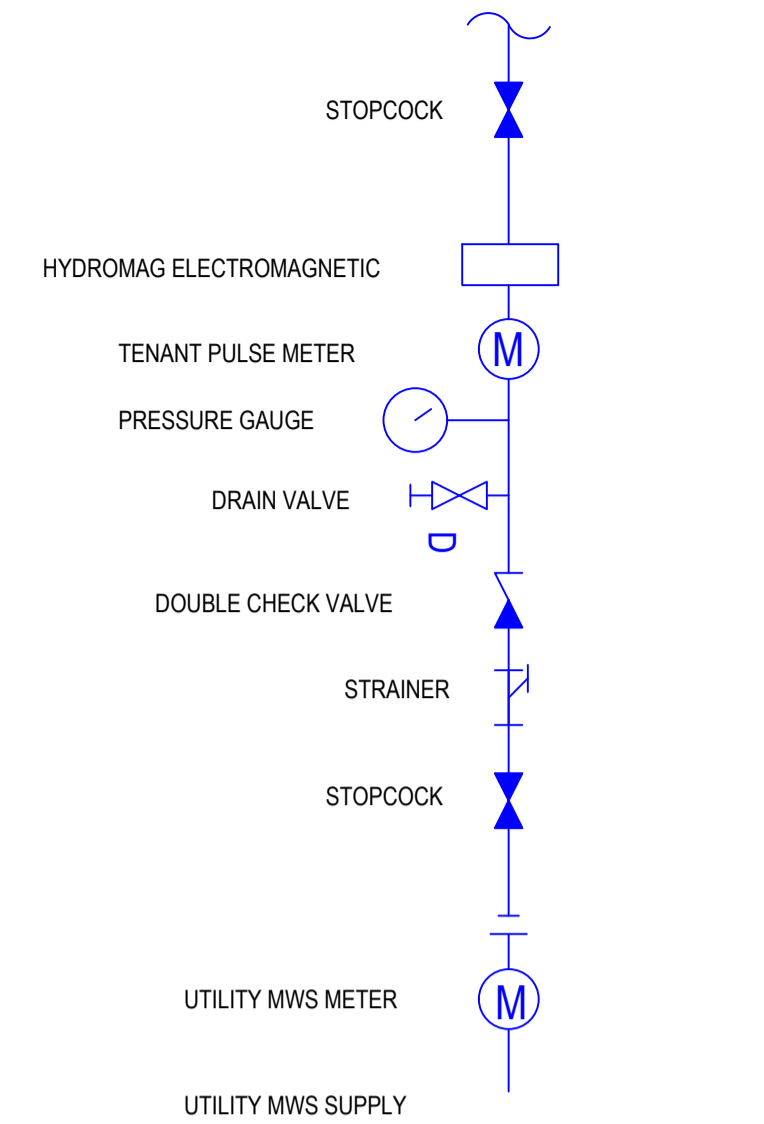
SCHEMATIC 4: VALVE ARRANGEMENT ON INCOMING LANDLORD SUPPLIES
