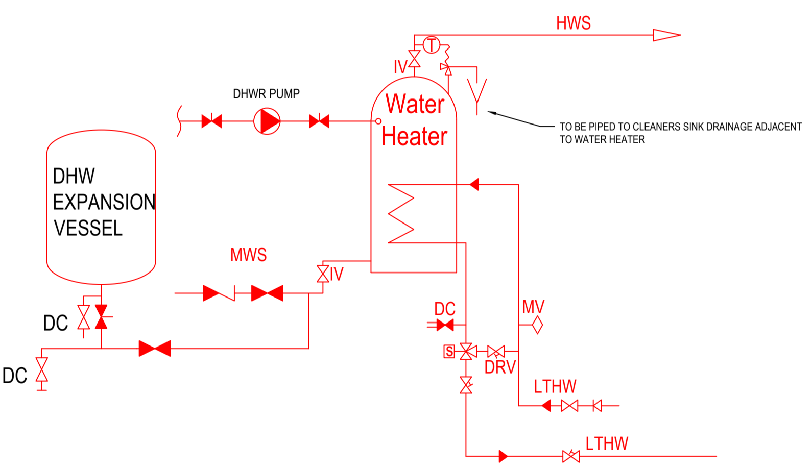
SCHEMATIC 5: TYPICAL CYLINDER DETAIL
