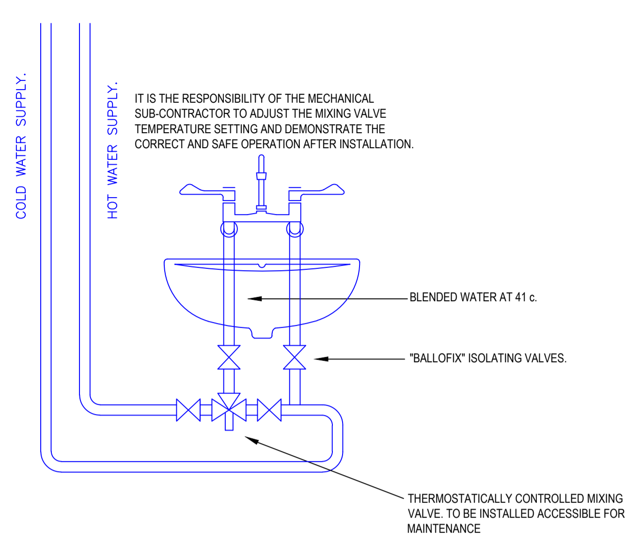
SCHEMATIC 3: THERMOSTATIC MIXING VALVE DETAIL
