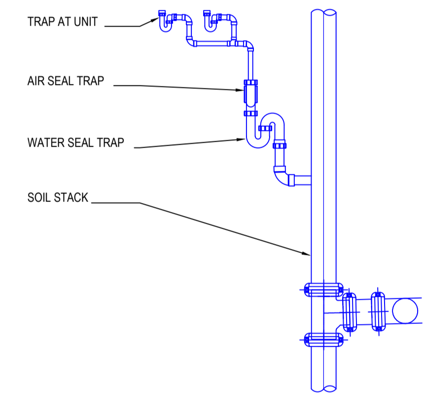
SCHEMATIC 11: TYPICAL CONDENSATE DETAIL
