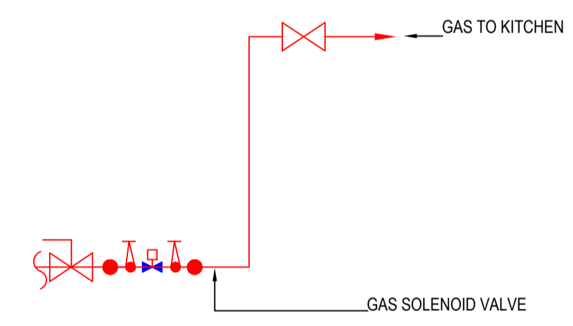
SCHEMATIC 10: GAS SCHEMATIC
