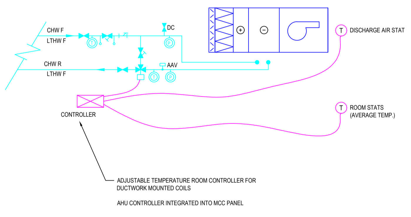
SCHEMATIC 6: TYPICAL HEATER BATTERY / COOLING COIL DETAIL
