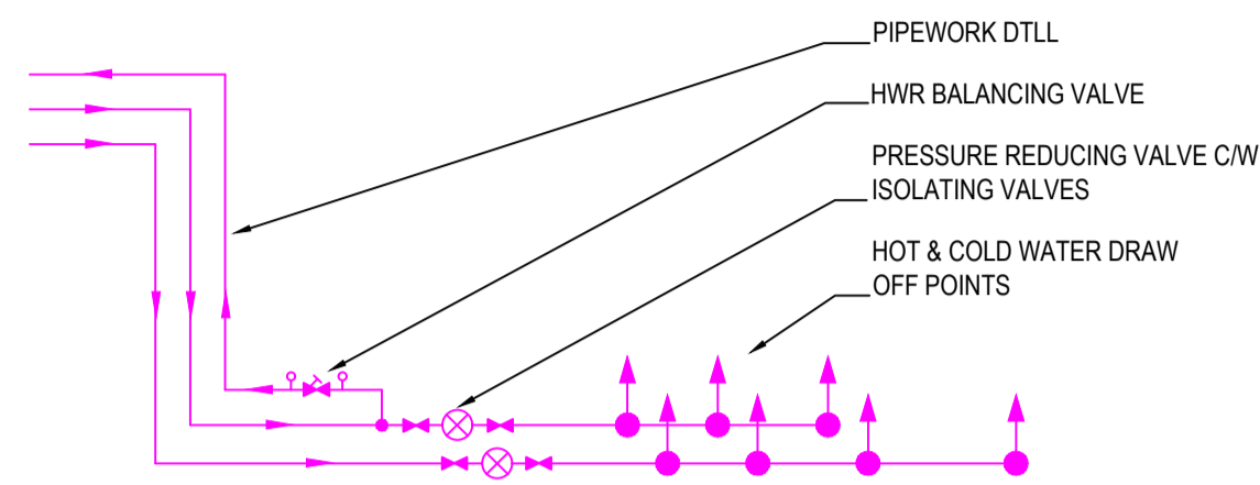
SCHEMATIC 2: THIS ARRANGEMENT SHALL BE PROVIDED FOR ALL H&CWS SINGLE OR MULTI-POINT DRAW-OFF POINTS
