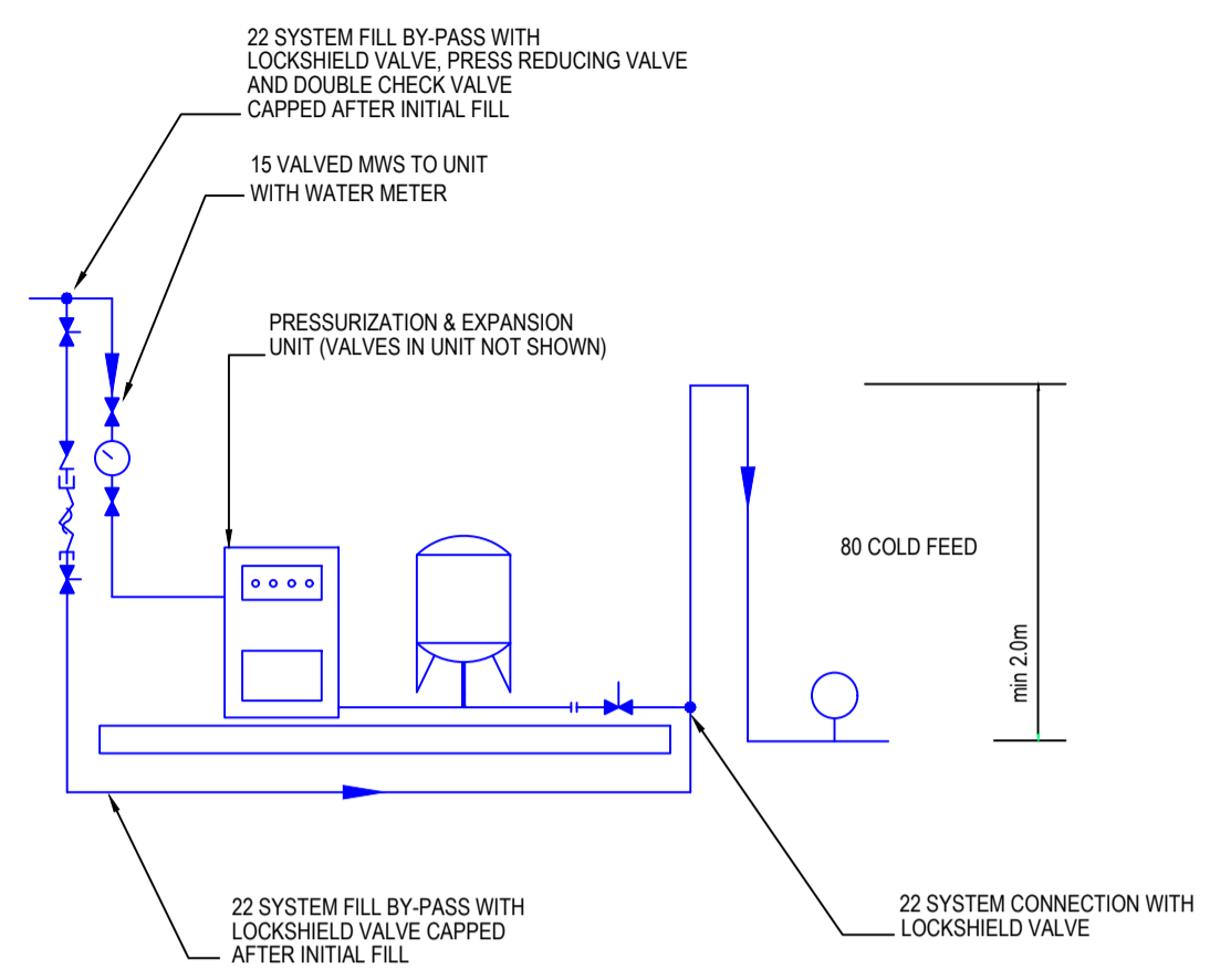
SCHEMATIC 1: PRESSURISATION UNIT ARRANGEMENT LPHW/CHW/COND. WATER
