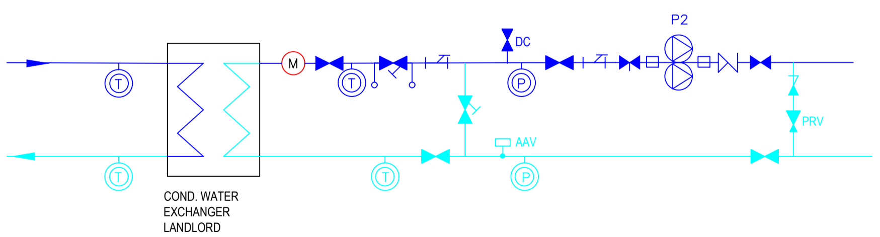
SCHEMATIC 9: COND. WATER CONNECTION TO LANDLORD SYSTEM
