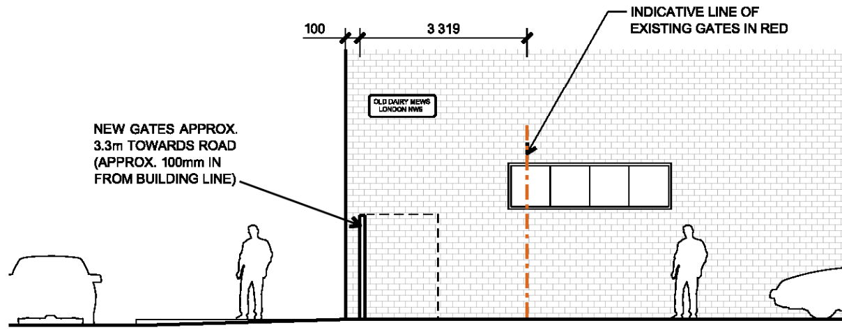
5 PROPOSED SECTION A 001 1:100 @ A3
