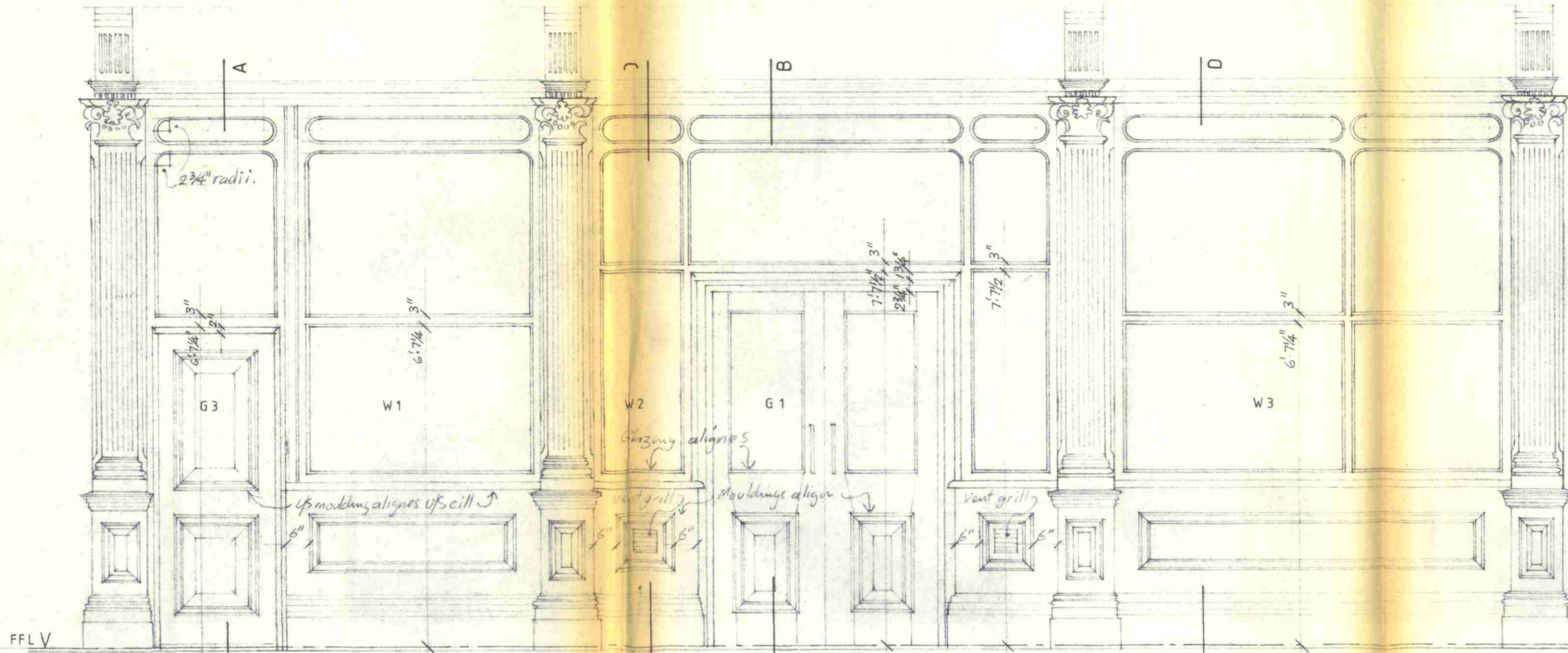
ELEVATION OF LOWER FRONT for sections AA to DD see drw 139126
