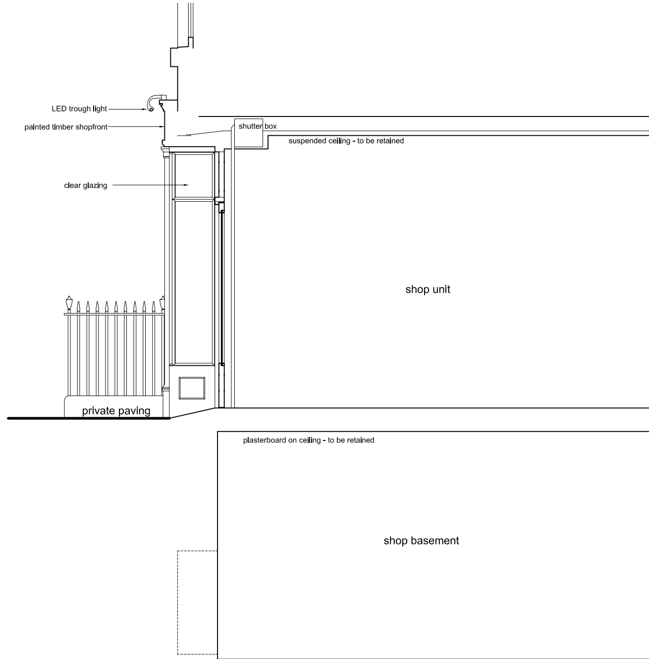
SECTION 0 1m
