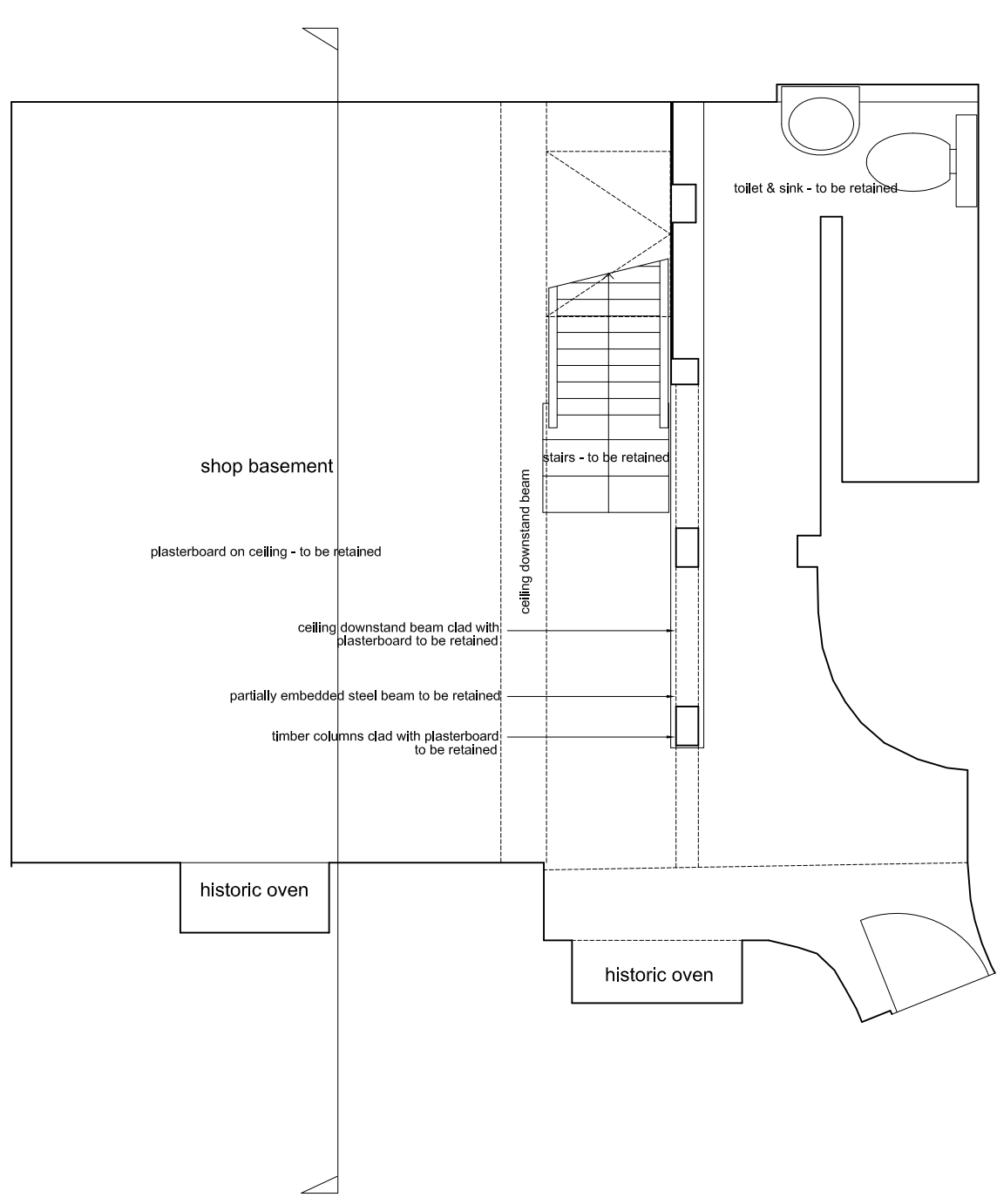
BASEMENT PLAN
