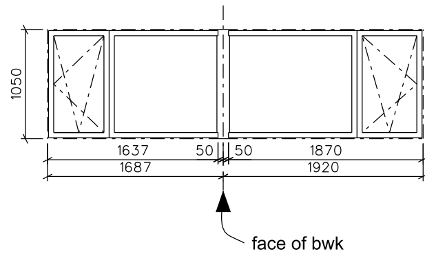
W2 KITCHEN CORNER WINDOW
