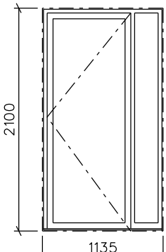
W5 DOOR outward opening
