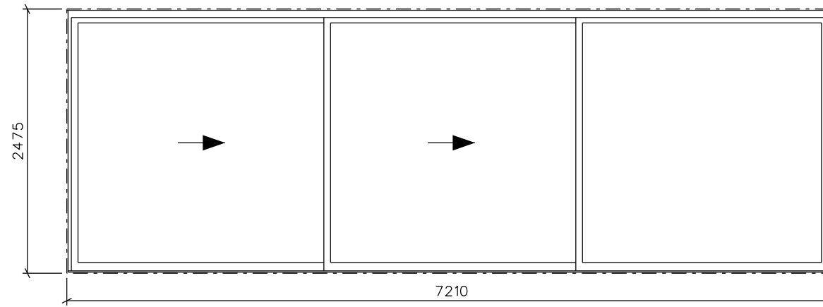
W3 THREE SECTION SLIDING DOOR
