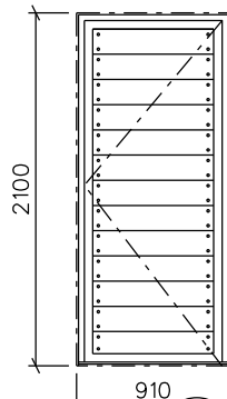
W4 DOOR outward opening with 150x15mm solid european oak boards to each face of 24mm WBP ply core
