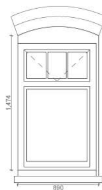
PROPOSED GROUND FLOOR WINDOW ELEVATION
