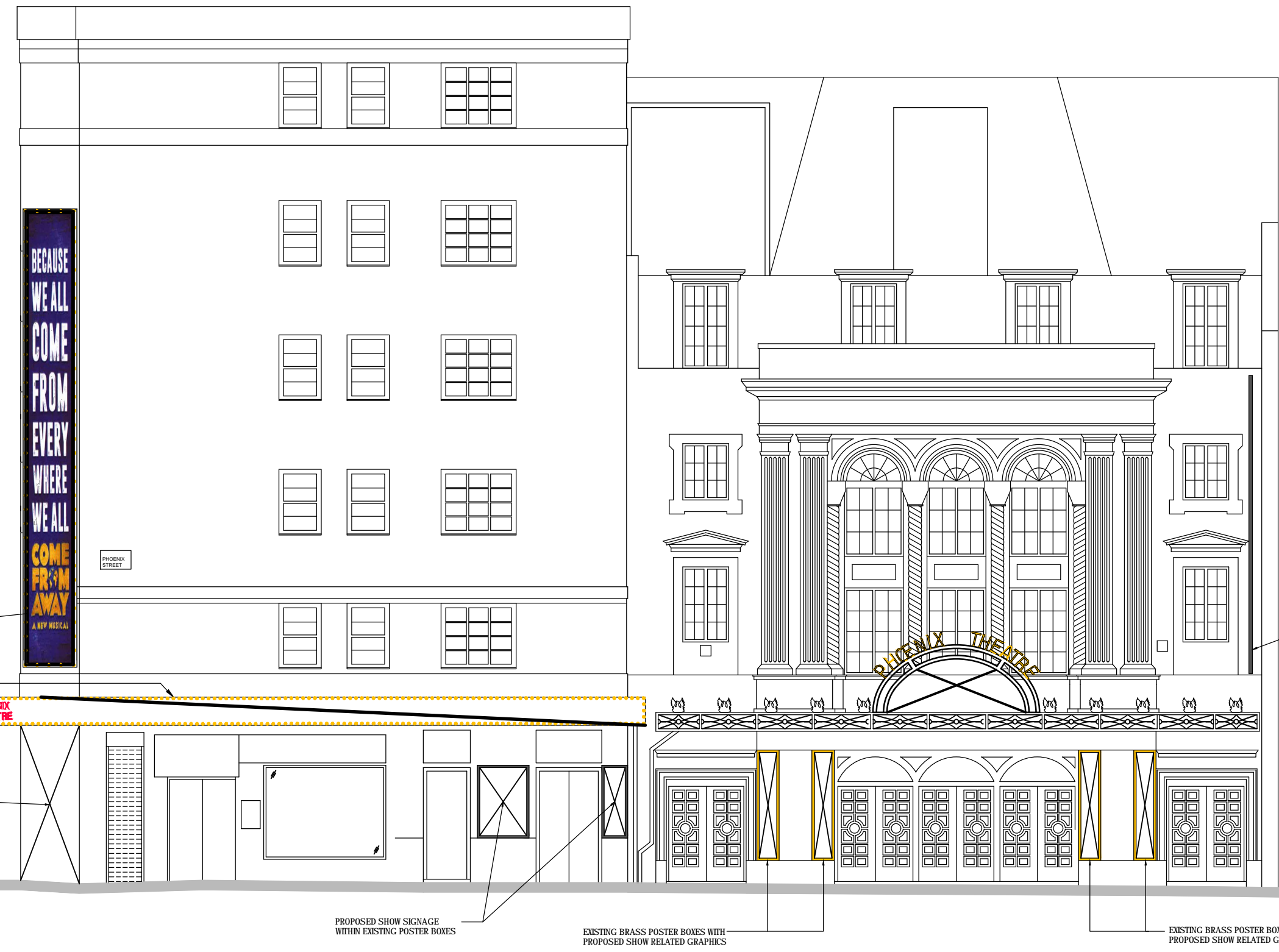
PROPOSED PHOENIX STREET ELEVATION (SCALE 1:50 AT A1)
