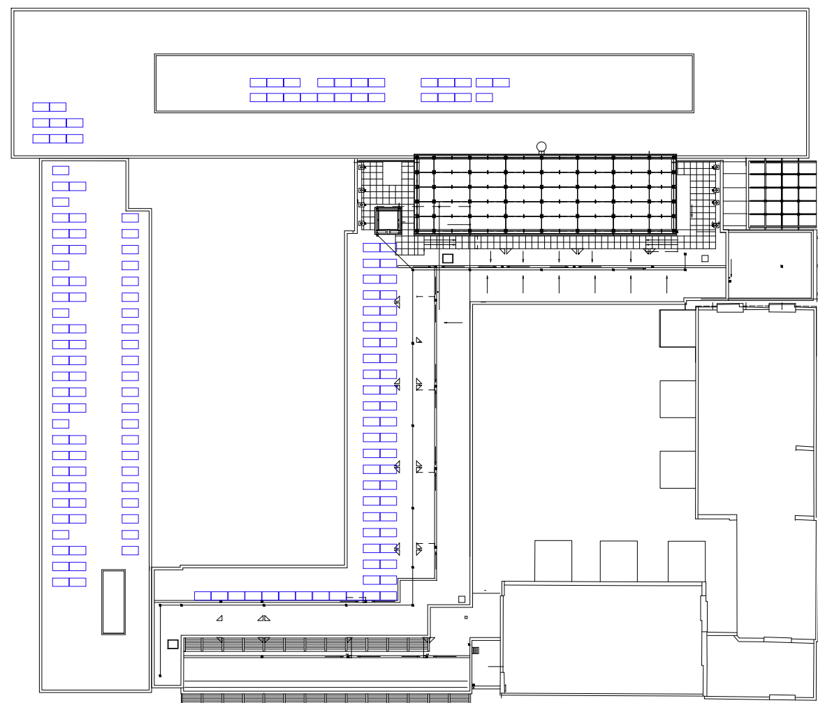
ROOF PLAN SHOWING PROPOSED PV PANEL LAYOUT
