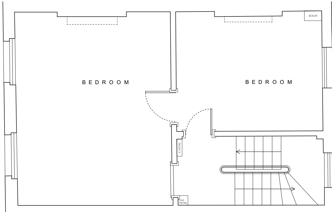
EXISTING SECOND FLOOR PLAN- SCALE 1:50
