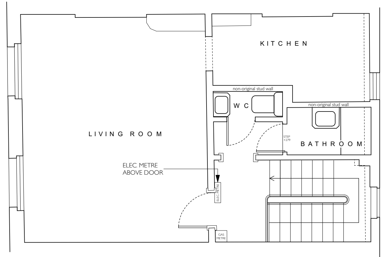
EXISTING THIRD FLOOR PLAN- SCALE 1:50
