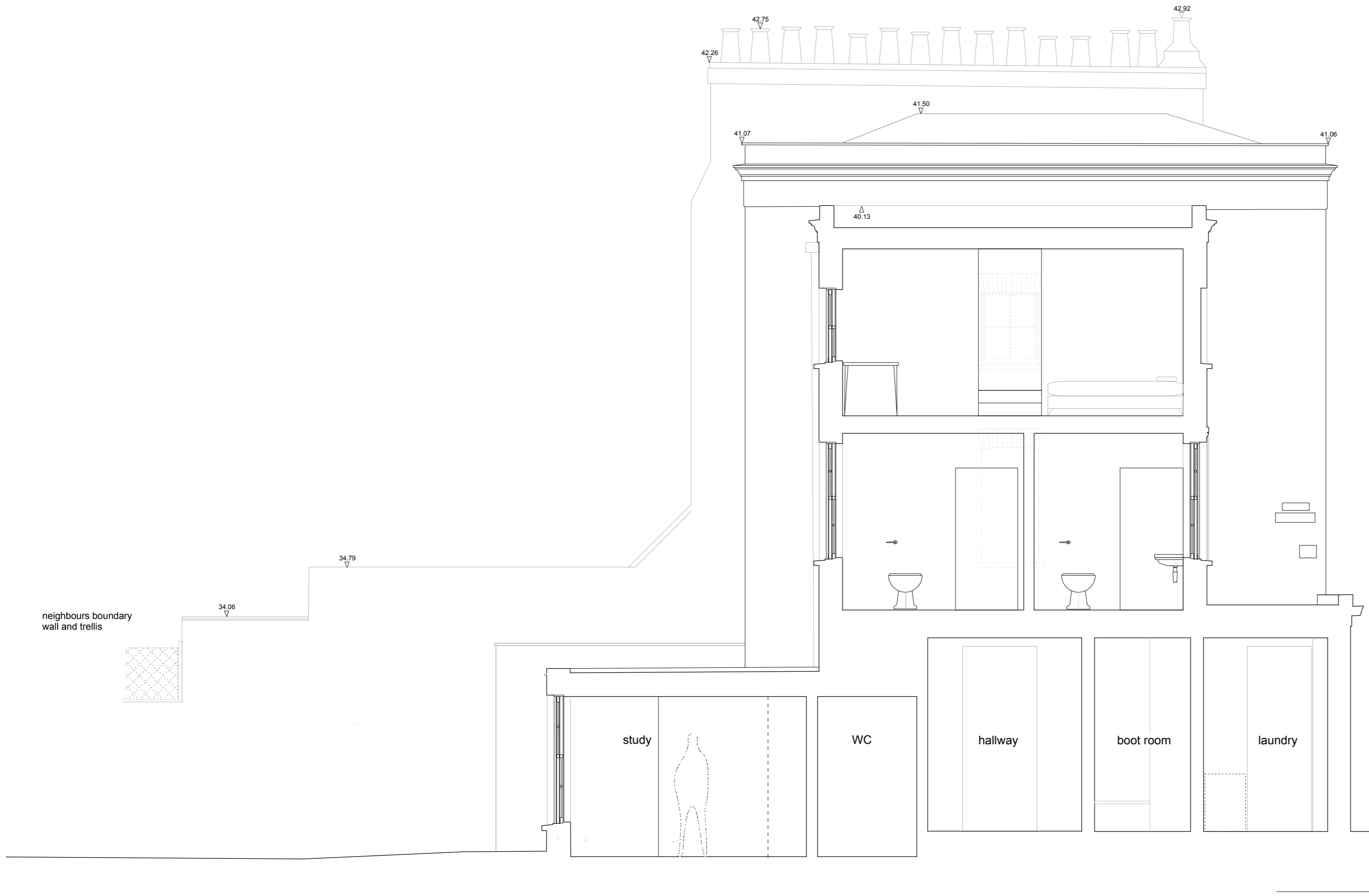
SECTION CC
