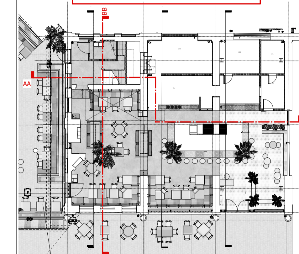
GROUND LEVEL PLAN 1:200
