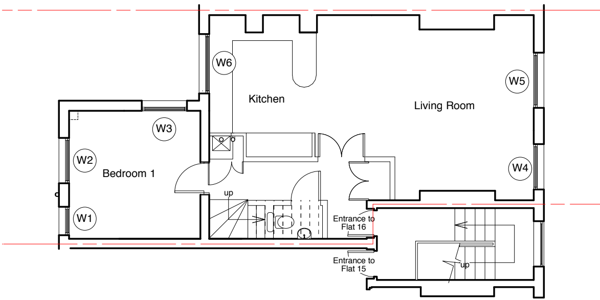
3rd Floor Plan as Existing scale 100
