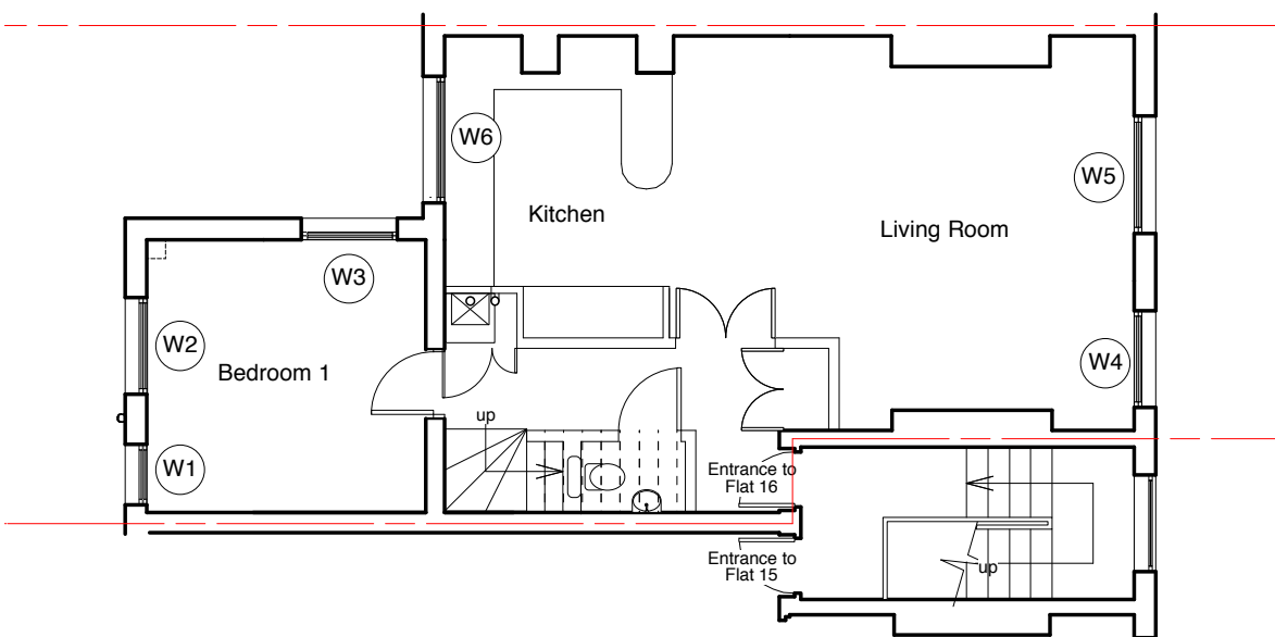
3rd Floor Plan as Proposed scale 100
