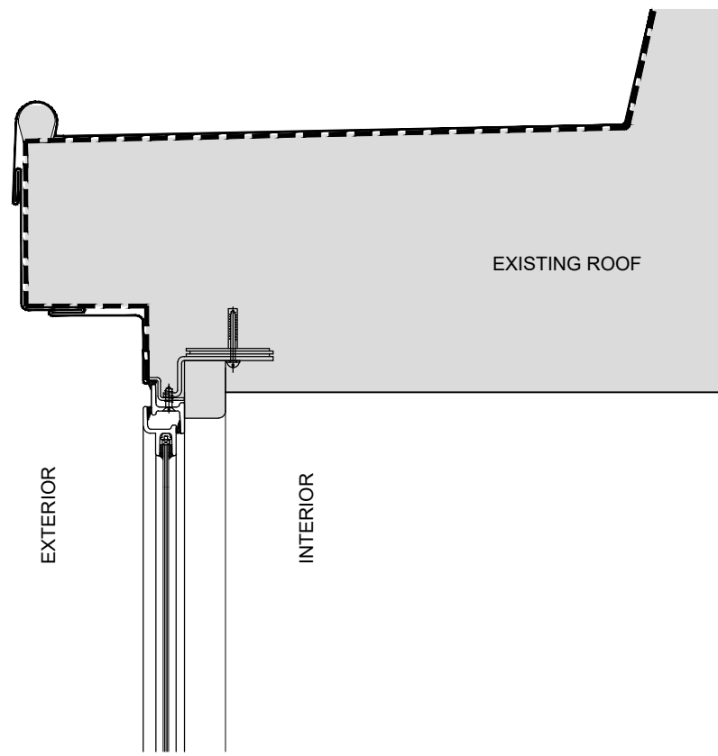
01 Dormer Window Head Detail- existing 1:5@ A1 / 1:10@ A3
