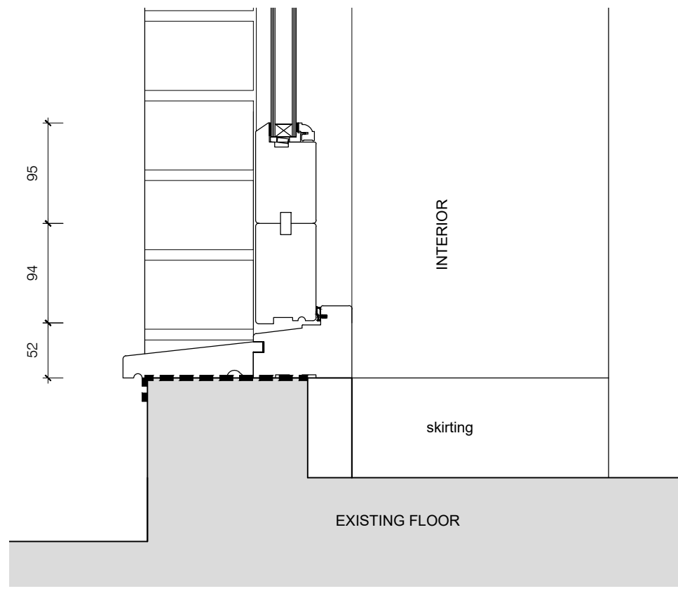
11 French Door Cill Detail- proposed 1:5@ A1 / 1:10@ A3
