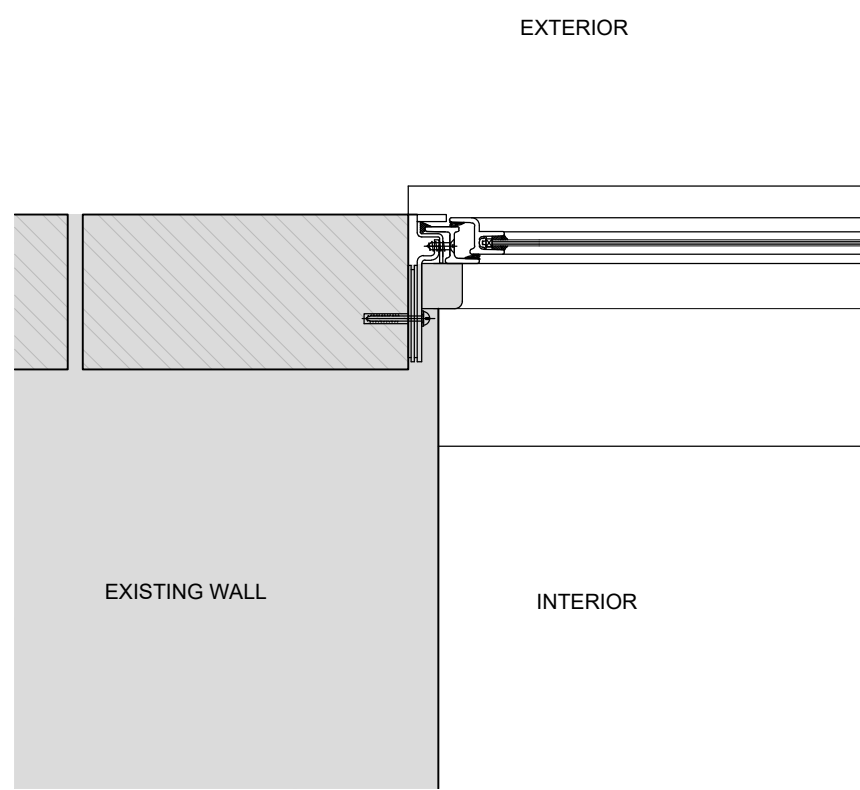
09 French Door Jamb Detail- existing 1:5@ A1 / 1:10@ A3
