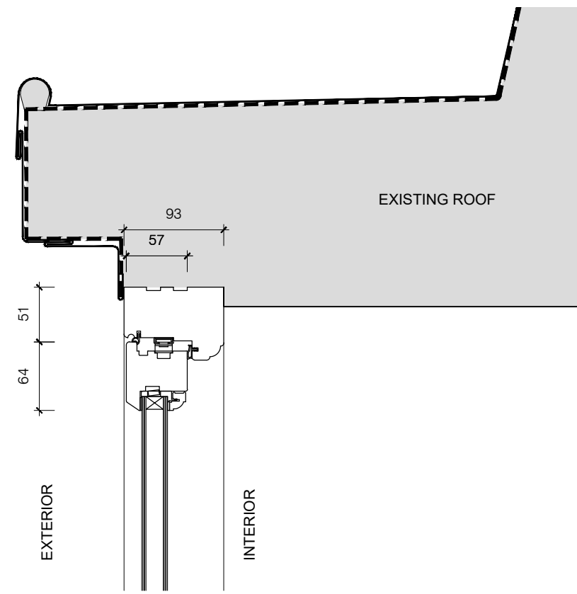
04 Dormer Window Head Detail- proposed 1:5@ A1 / 1:10@ A3
