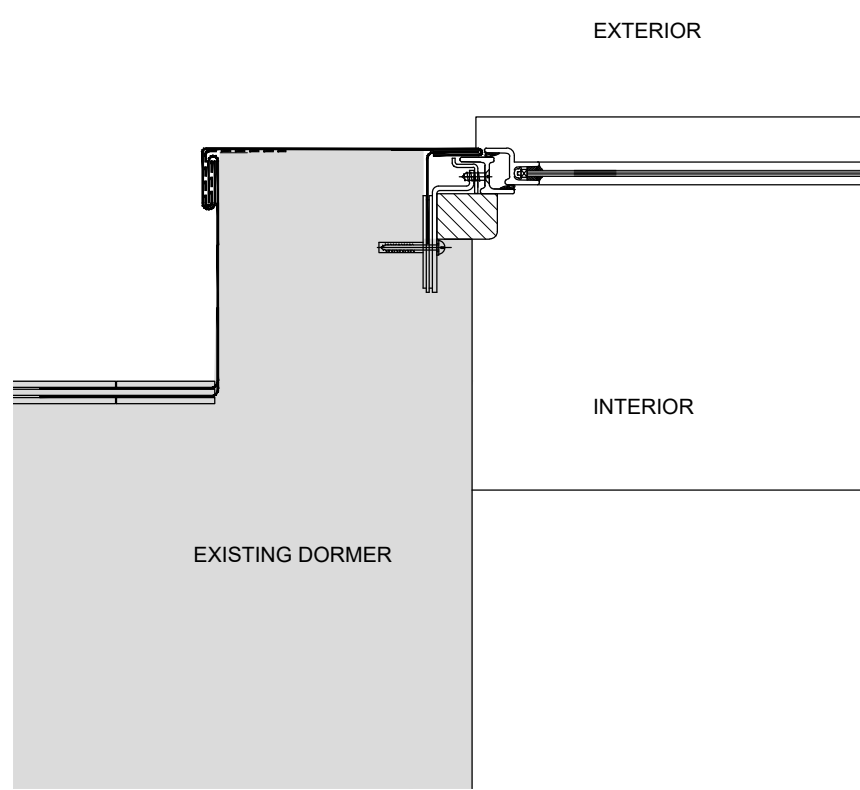
03 Dormer Window Jamb Detail- existing 1:5@ A1 / 1:10@ A3
