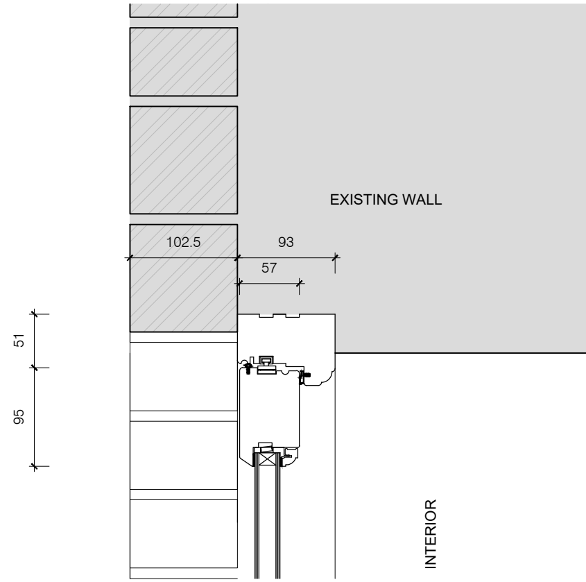
10 French Door Head Detail- proposed 1:5@ A1 / 1:10@ A3
