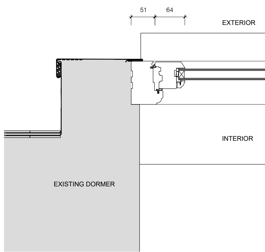
06 Dormer Jamb Detail- proposed 1:5@ A1 / 1:10@ A3
