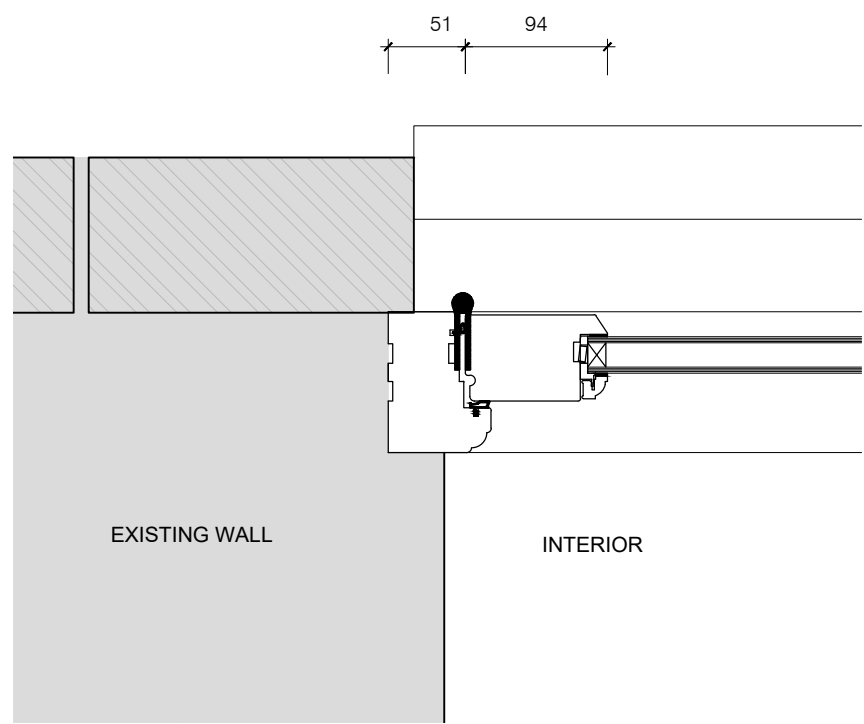
12 French Door Jamb Detail- proposed 1:5@ A1 / 1:10@ A3
