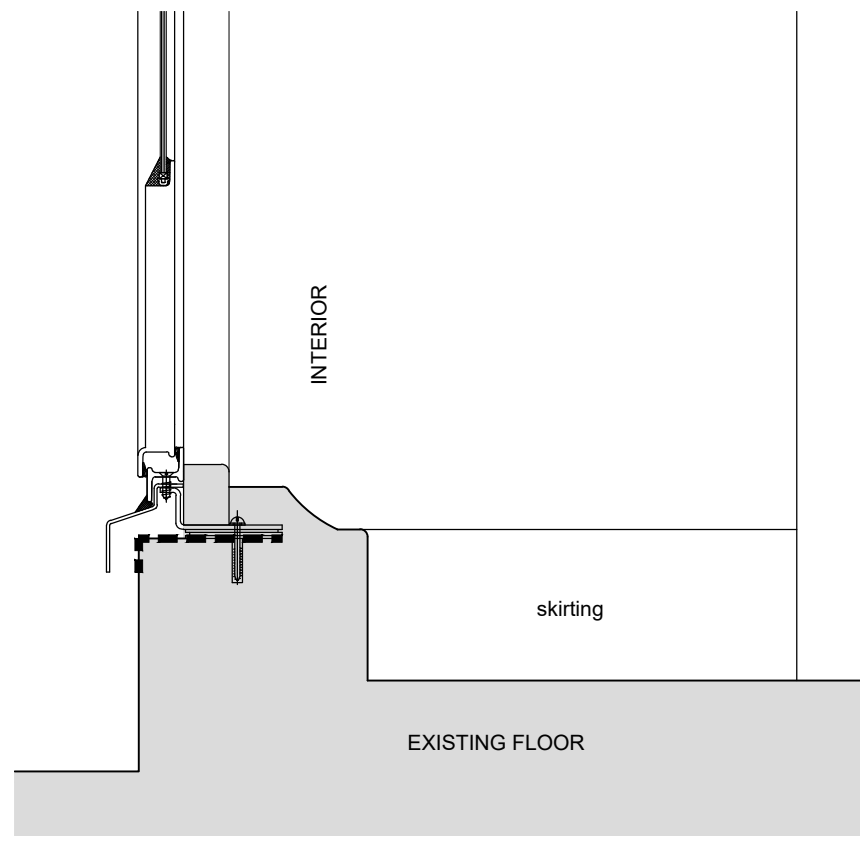
08 French Door Cill Detail- existing 1:5@ A1 / 1:10@ A3
