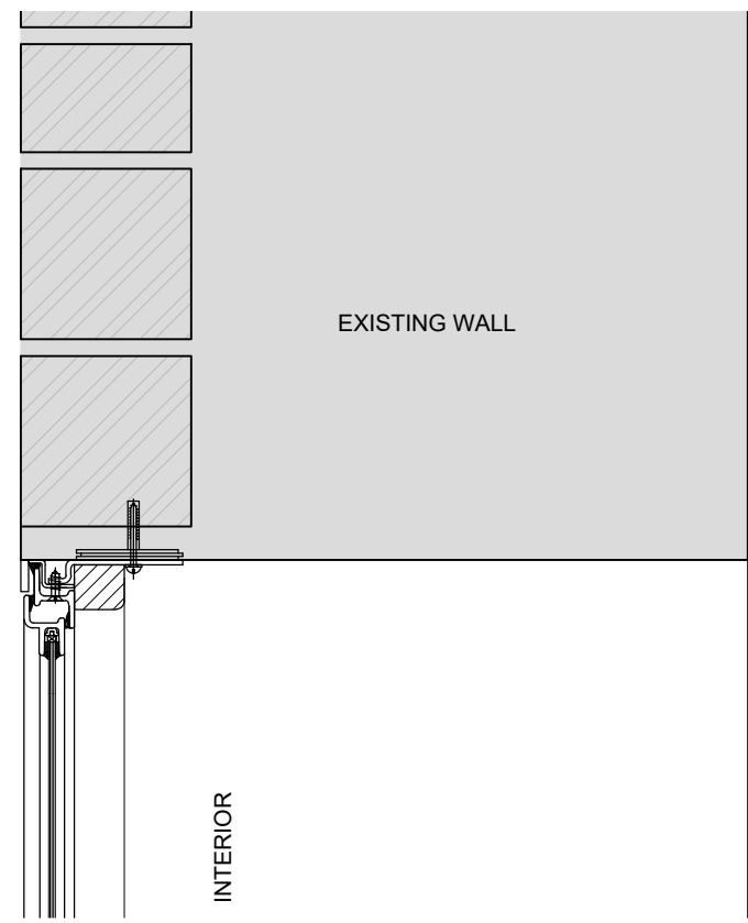
07 French Door Head Detail- existing 1:5@ A1 / 1:10@ A3
