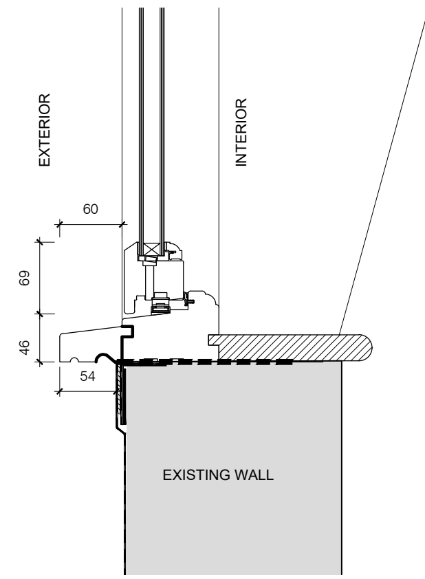
05 Dormer Window Cill Detail- proposed 1:5@ A1 / 1:10@ A3
