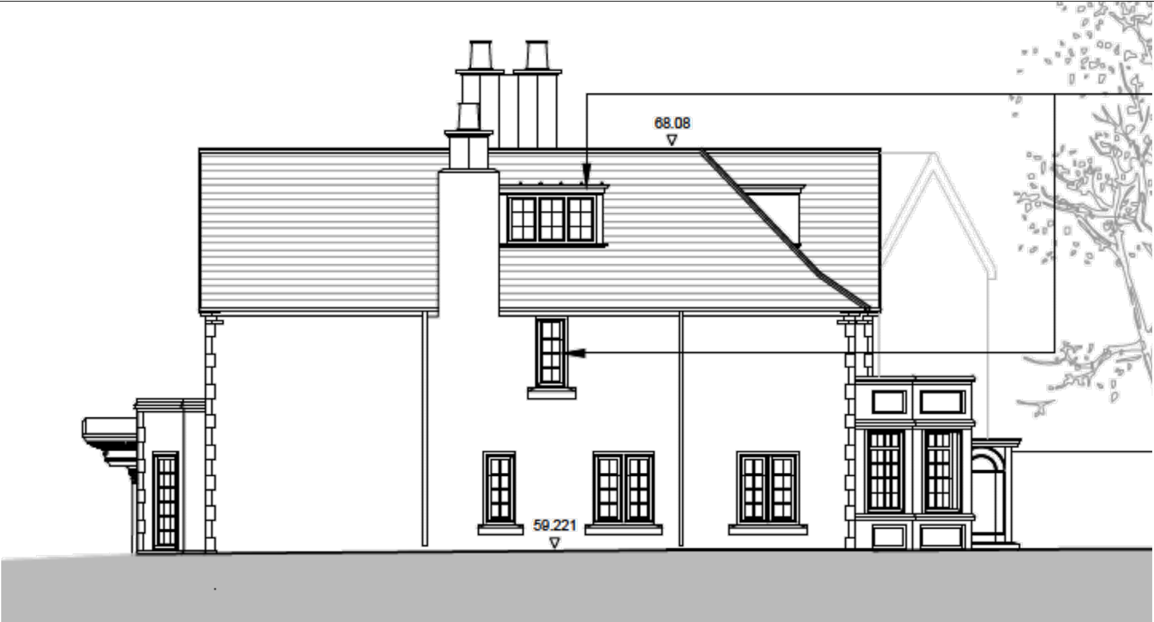
Consented Flank Elevation (2015/6106/P) Scale 1:50
