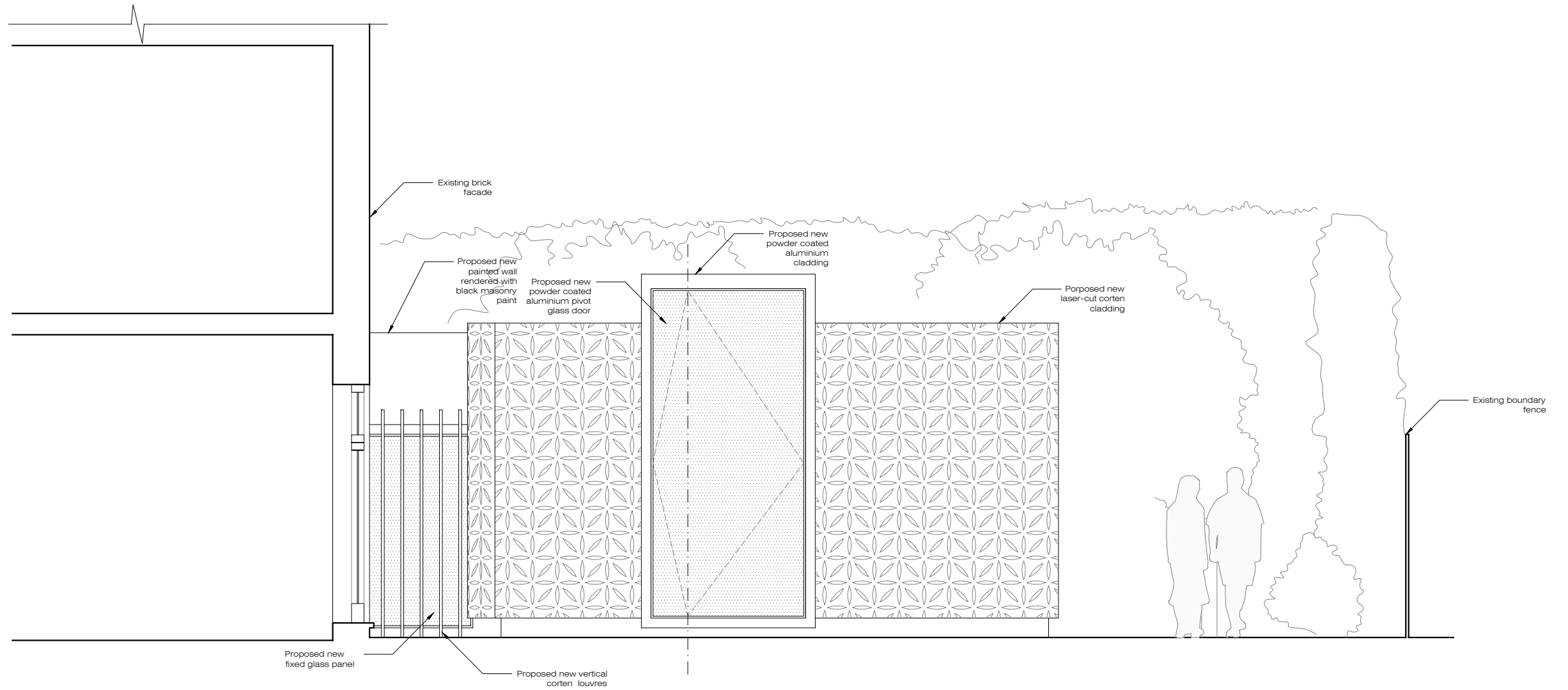
01 Proposed Elevation AA' scale: 1:50
