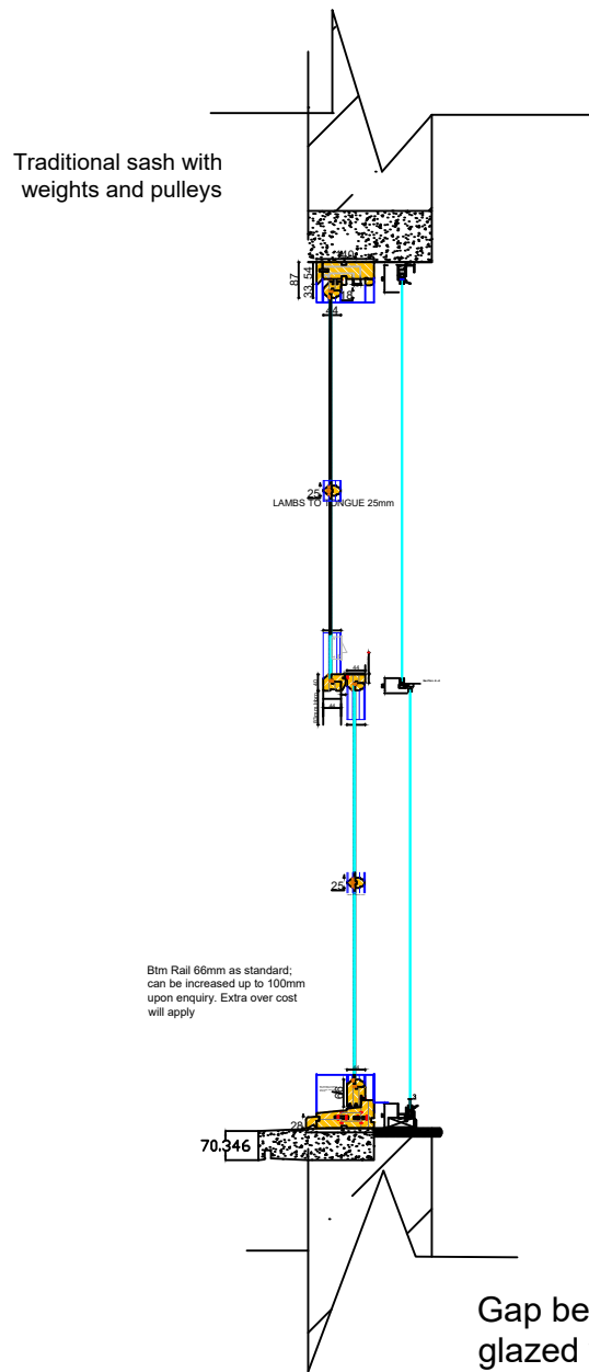
Window Section A-A
