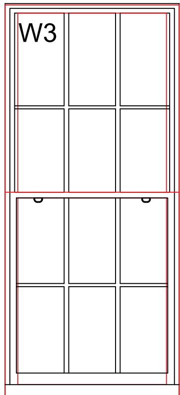
Window from inside with Secondary glazing
