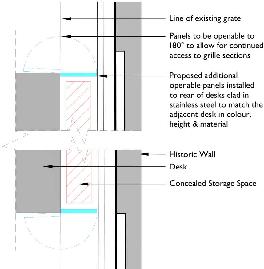
5 200 Proposed Desk Alteration 1:50 @ A3
