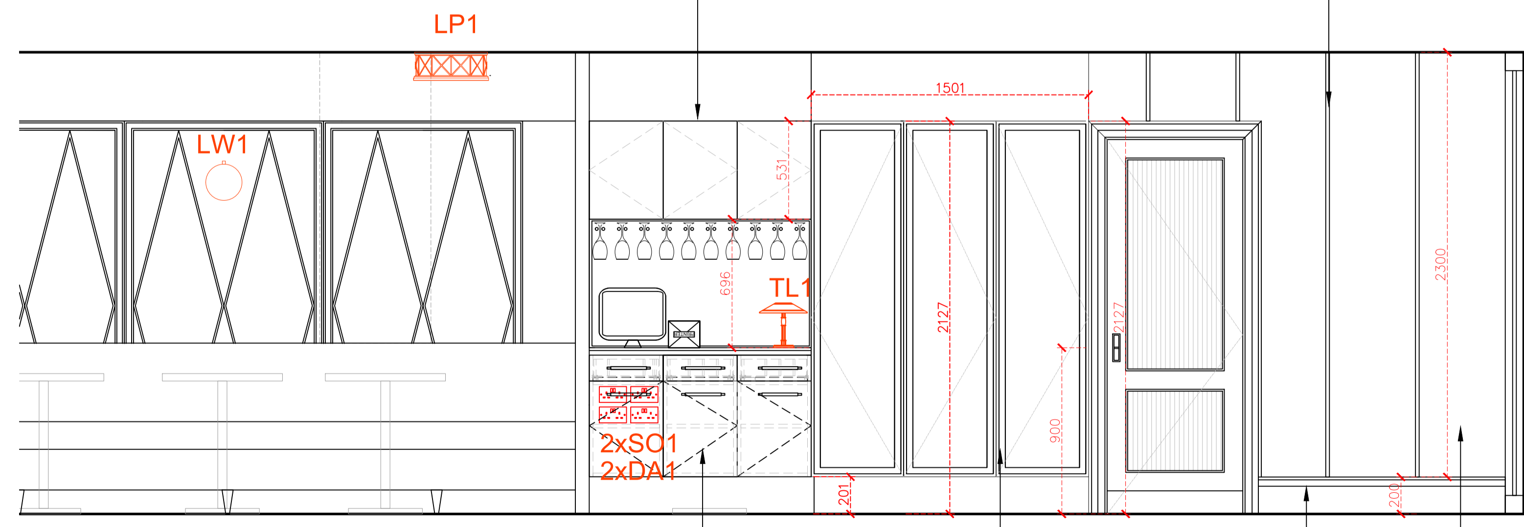
1 Elevation B Scale 1:20@A1
