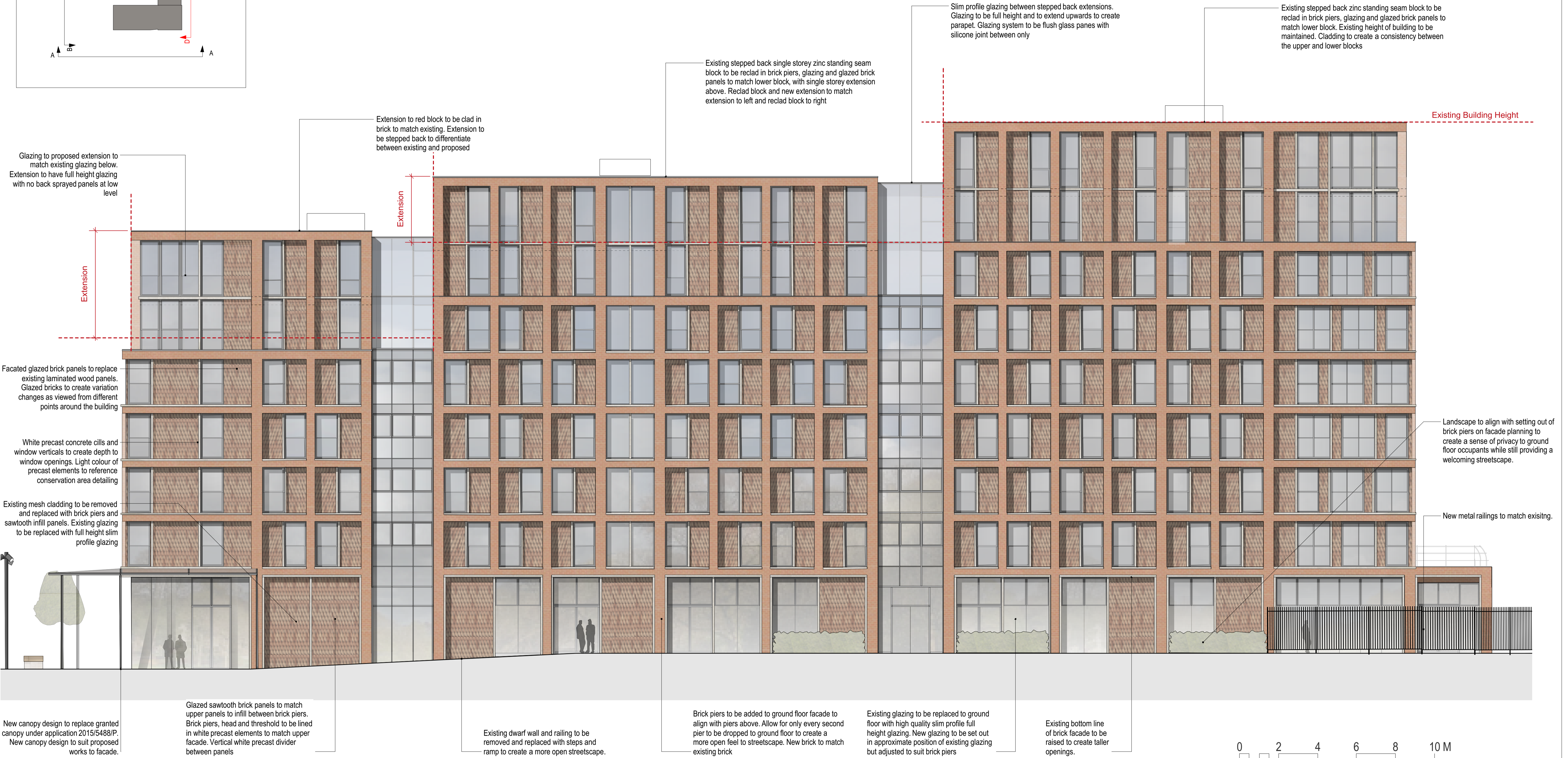
01 Proposed East Elevation Scale 1 : 200 @ A3
