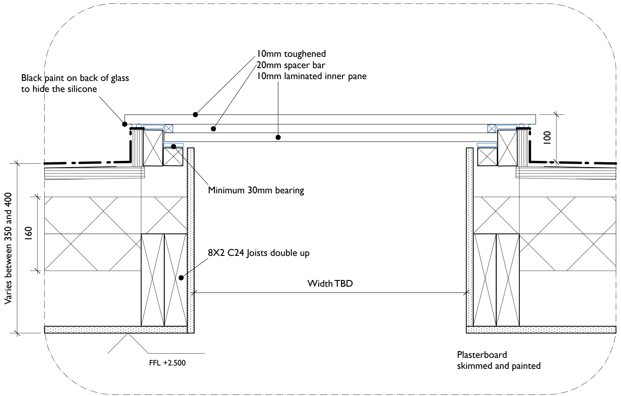
Warm roof construction
