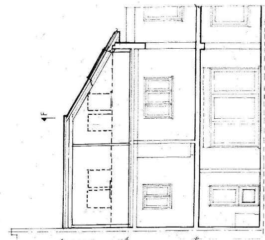
Section G-G
