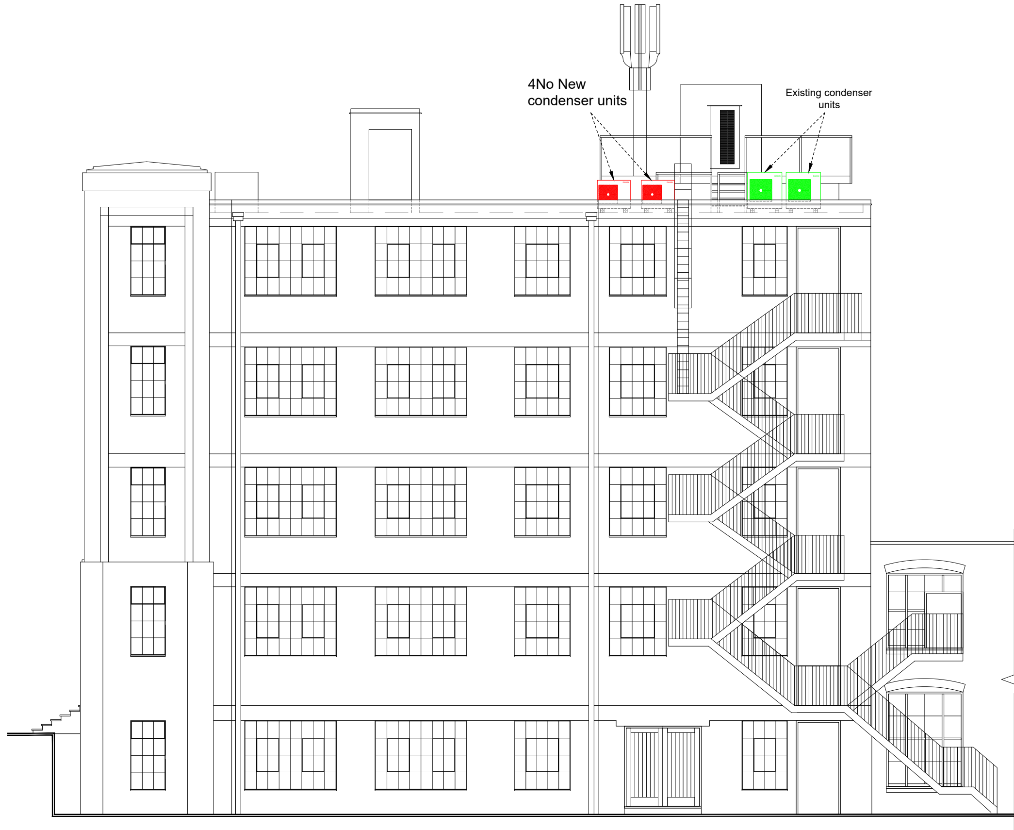
Proposed South Elevation (Facing Rotunda Building)
