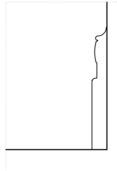
SKIRTING (LIVING ROOM AND KITCHEN) SCALE 1:5
