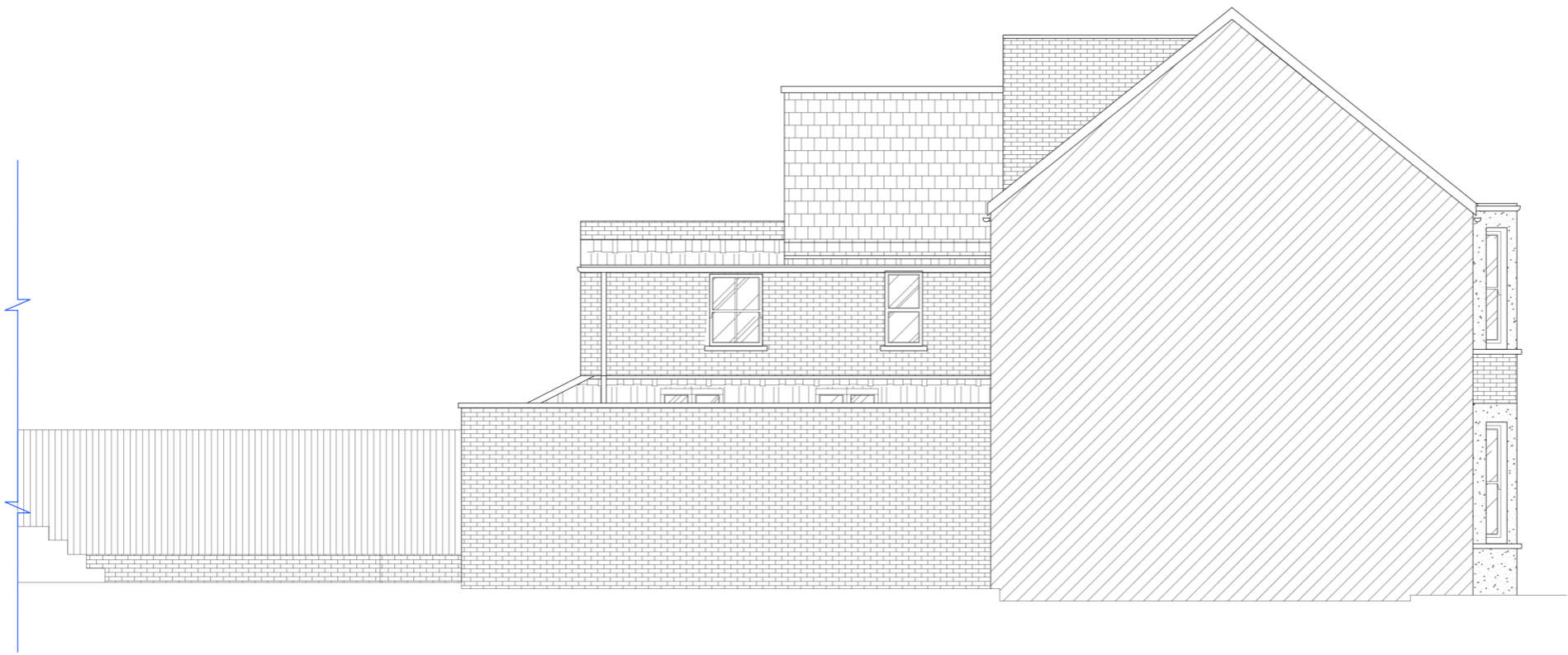
CONSTRUCTED SIDE ELEVATION 0 1 2 3 4 5m
