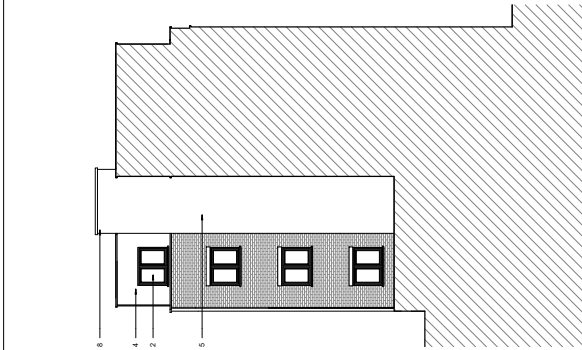
Rear Elevation as Proposed (3-3) 1:100
