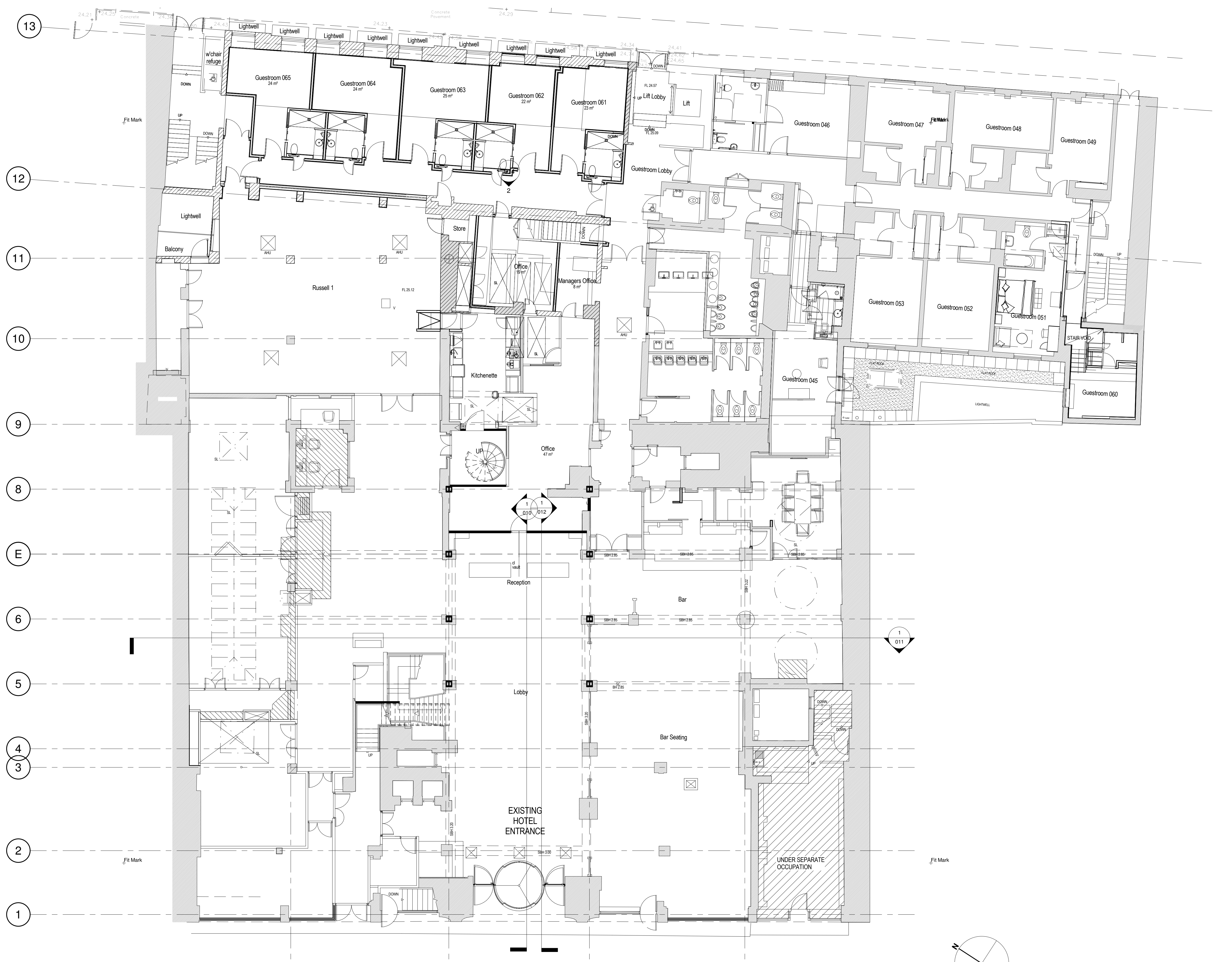
Ground Floor as Proposed 1 : 100
