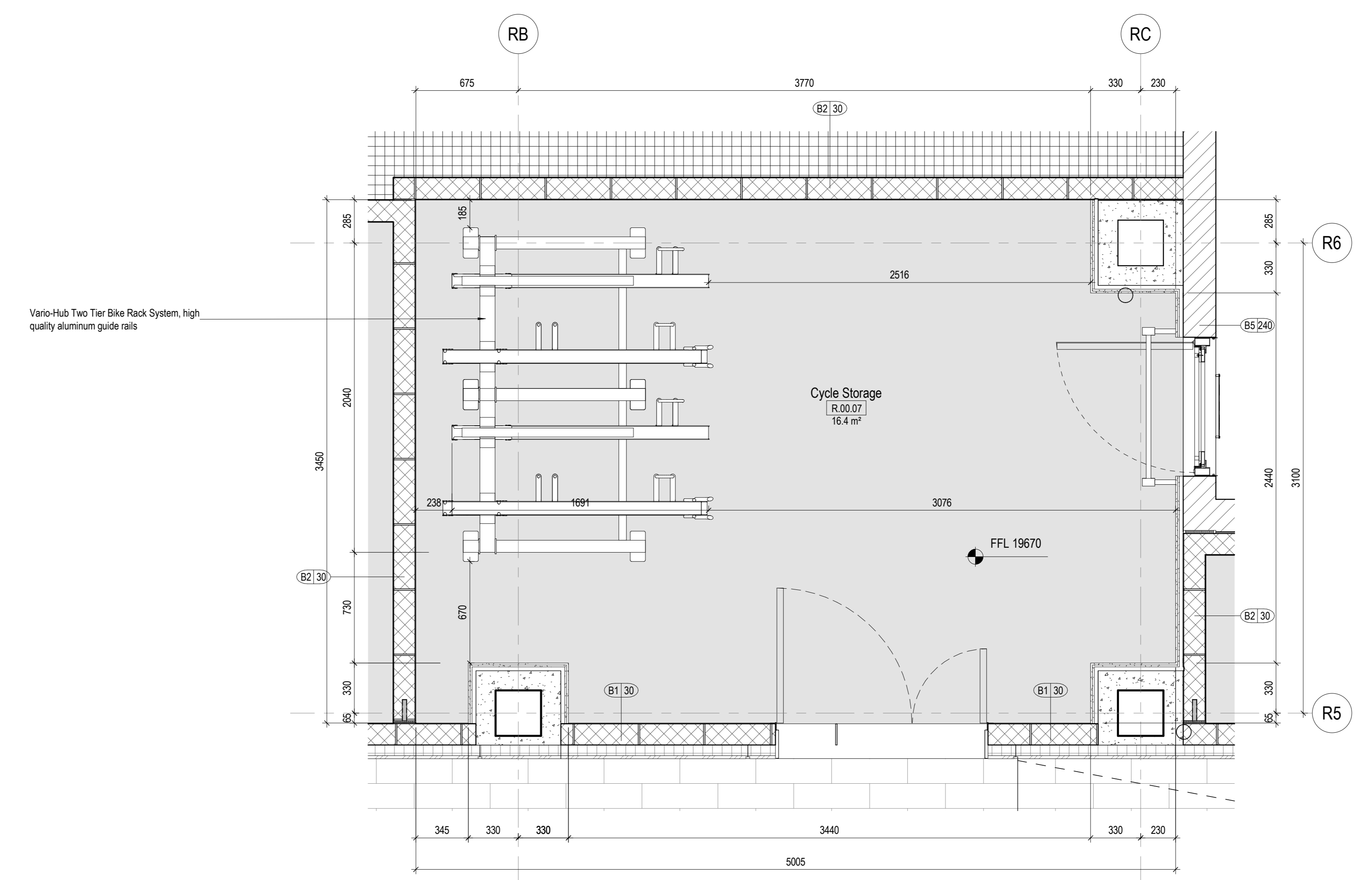
1 Cycle Store 2 - Enlarged Plan 1:20
