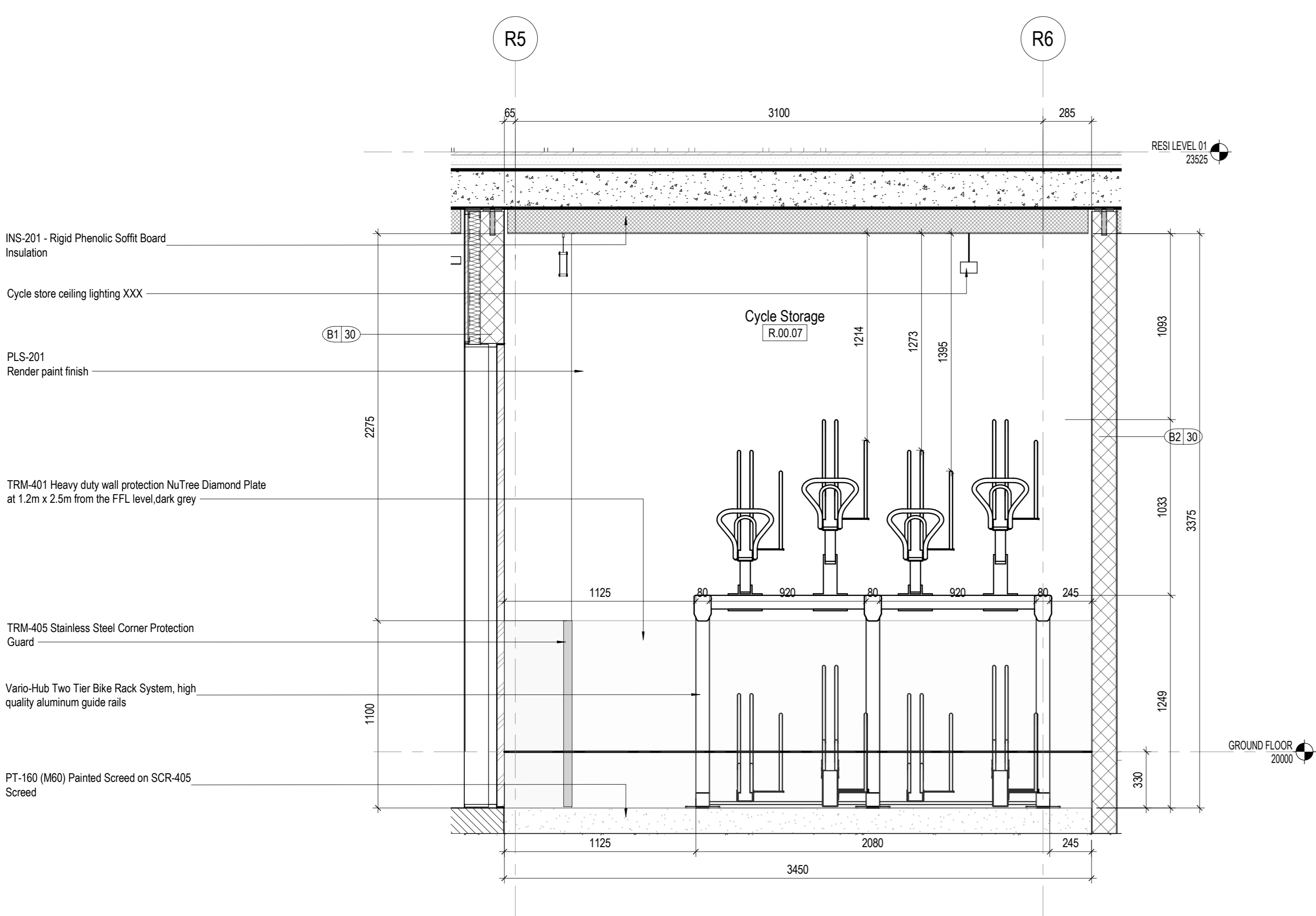
2 Cycle Store 2 - Enlarged Short Section 1:20
