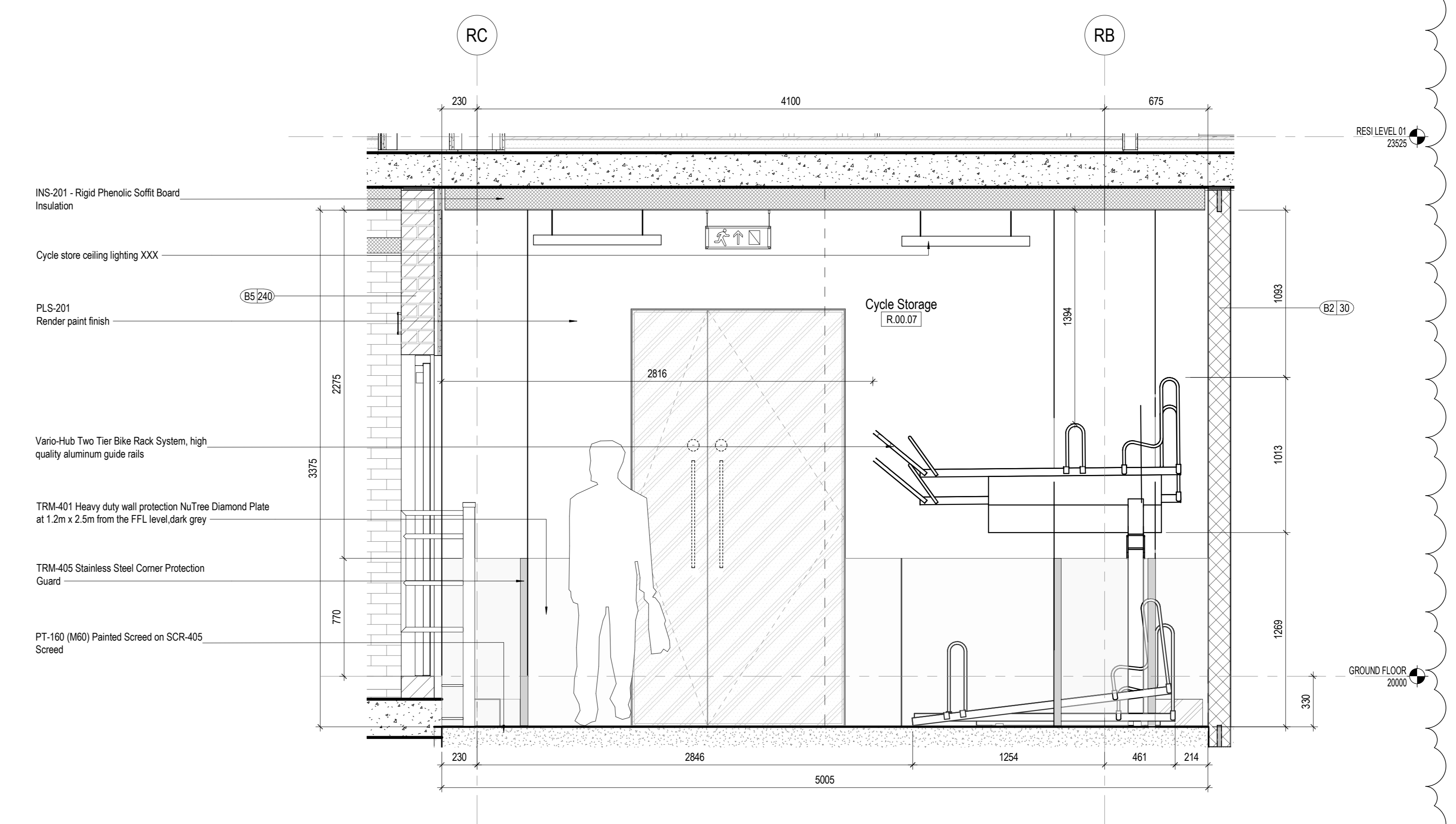
3 Cycle Store 2 - Enlarged Long Section 1:20
