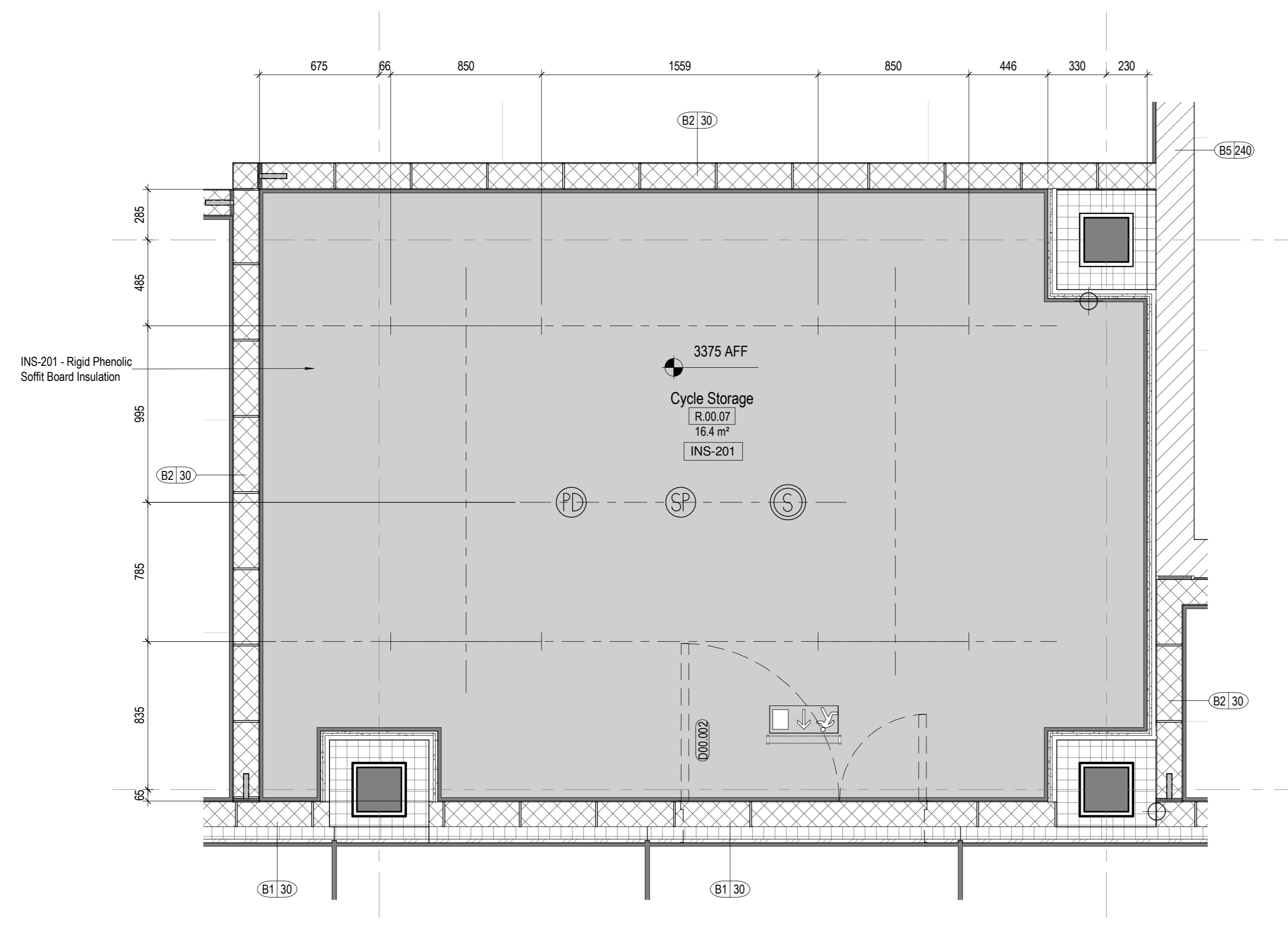
4 Cycle Store 2 - Enlarged RCP Plan 1:20
