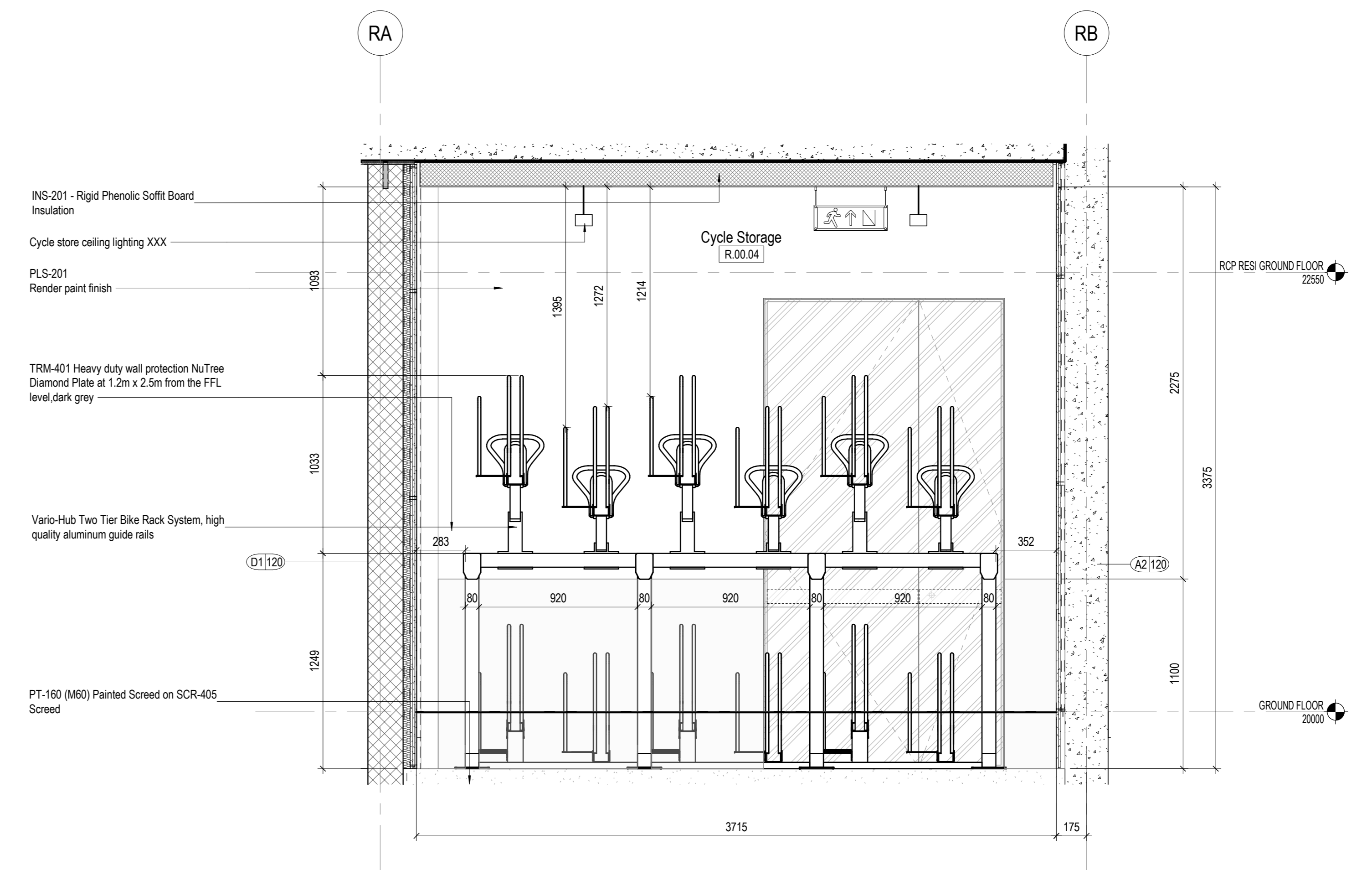
5 Cycle Store 1 - Enlarged Short Section 1:20
