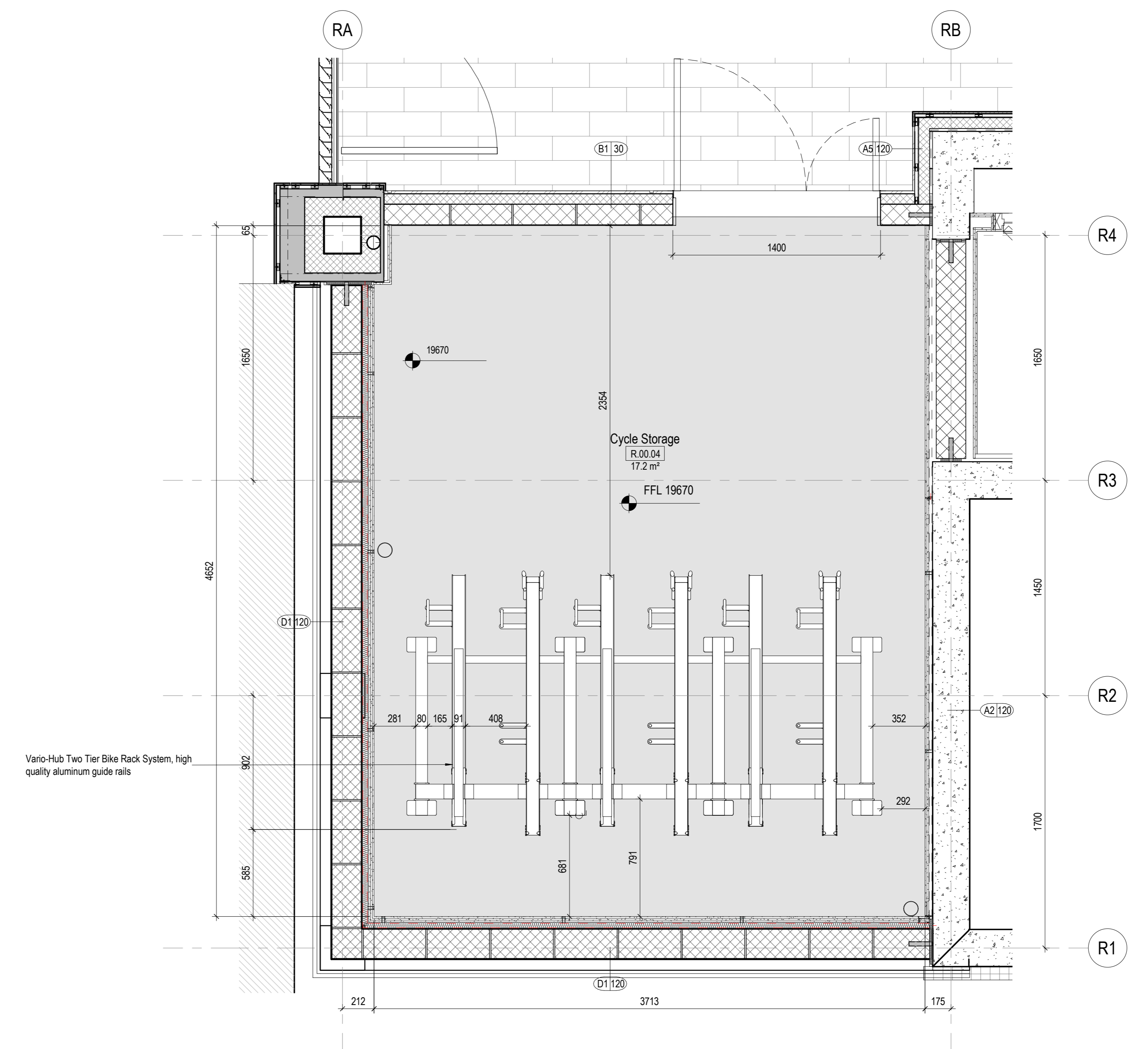
1 Cycle Store 1 - Enlarged Plan 1:20
