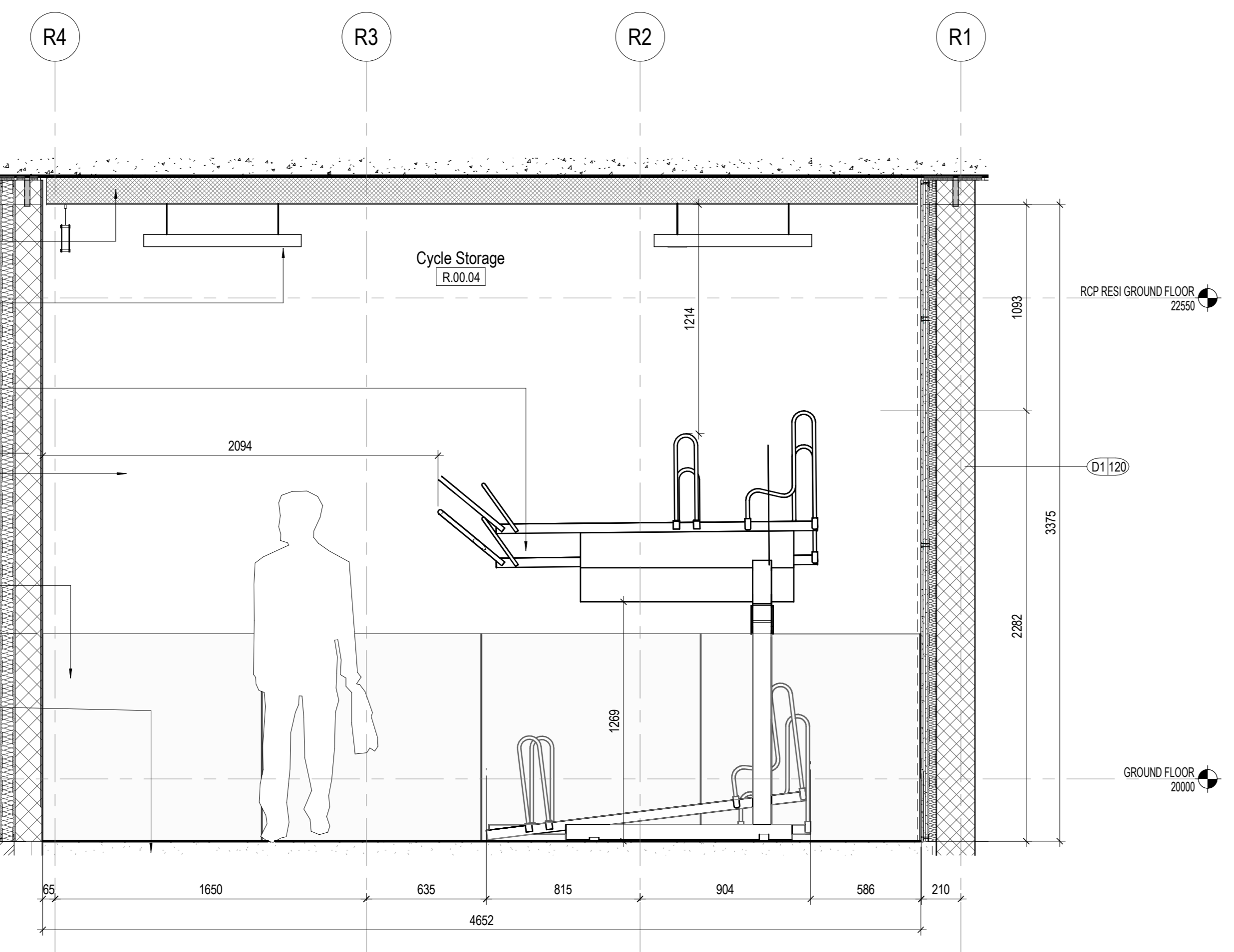
2 Cycle Store 1 - Enlarged Long Section 1:20
