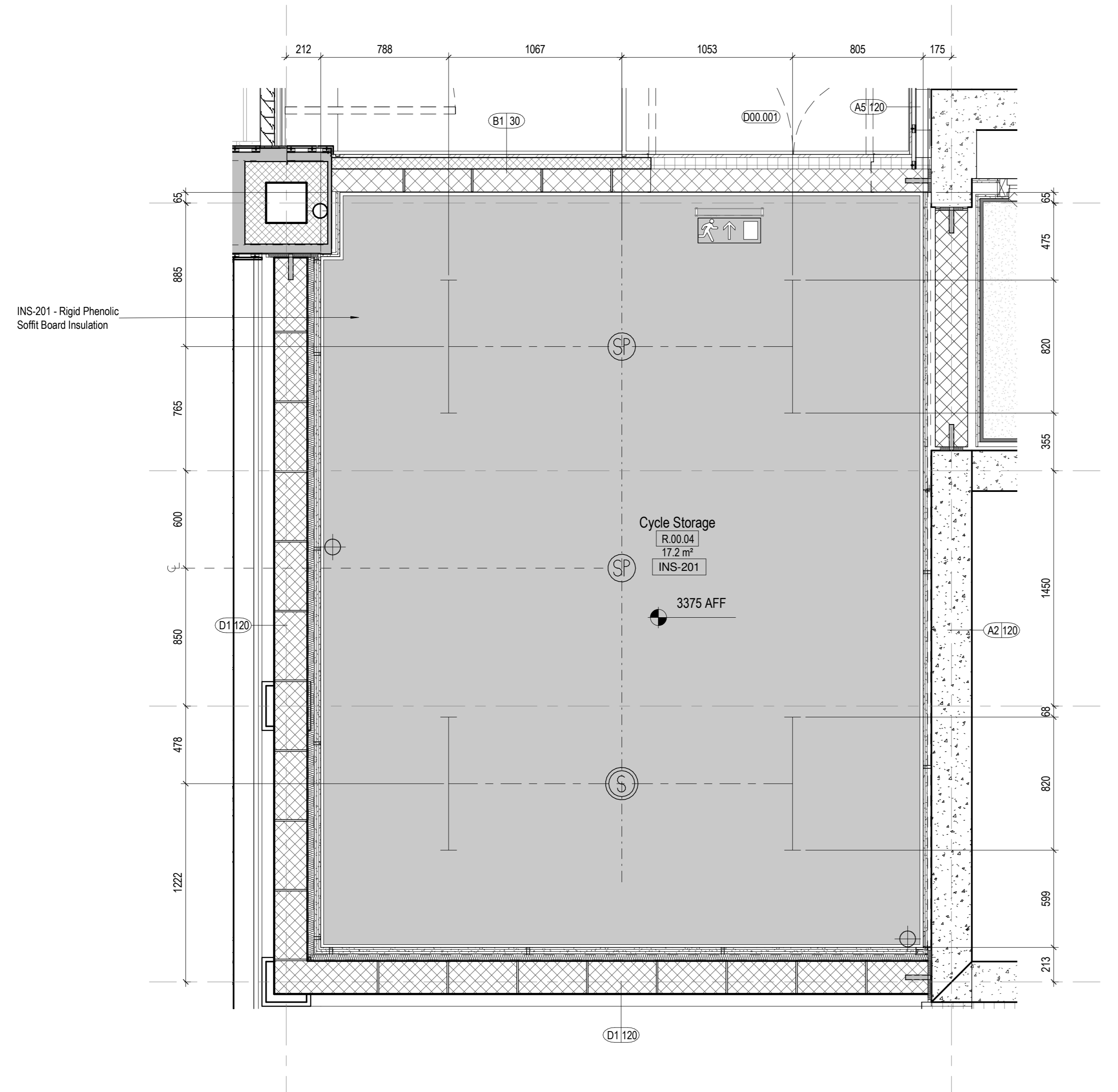
3 Cycle Store 1 - Enlarged RCP Plan 1:20
