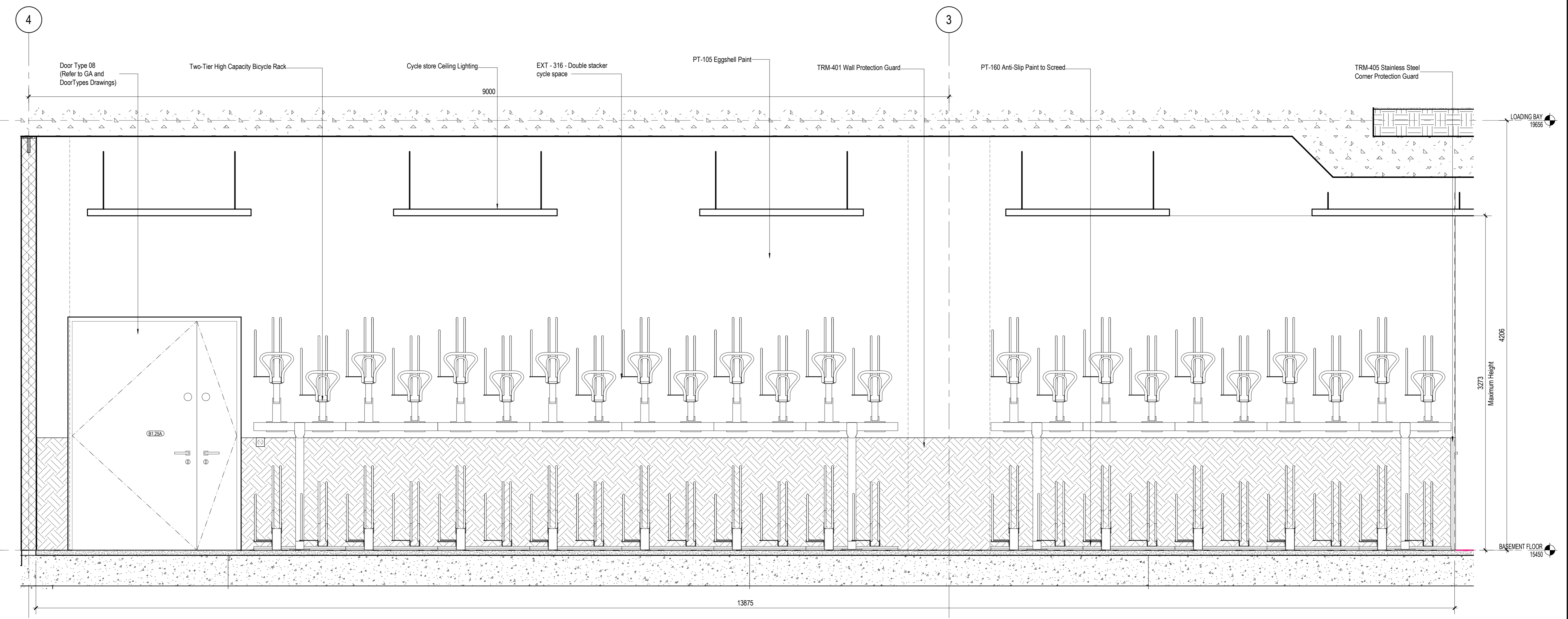
③ Cycle Parking 3 - Enlarged Elevation 1 1:20 Referencing View: 2/A0
