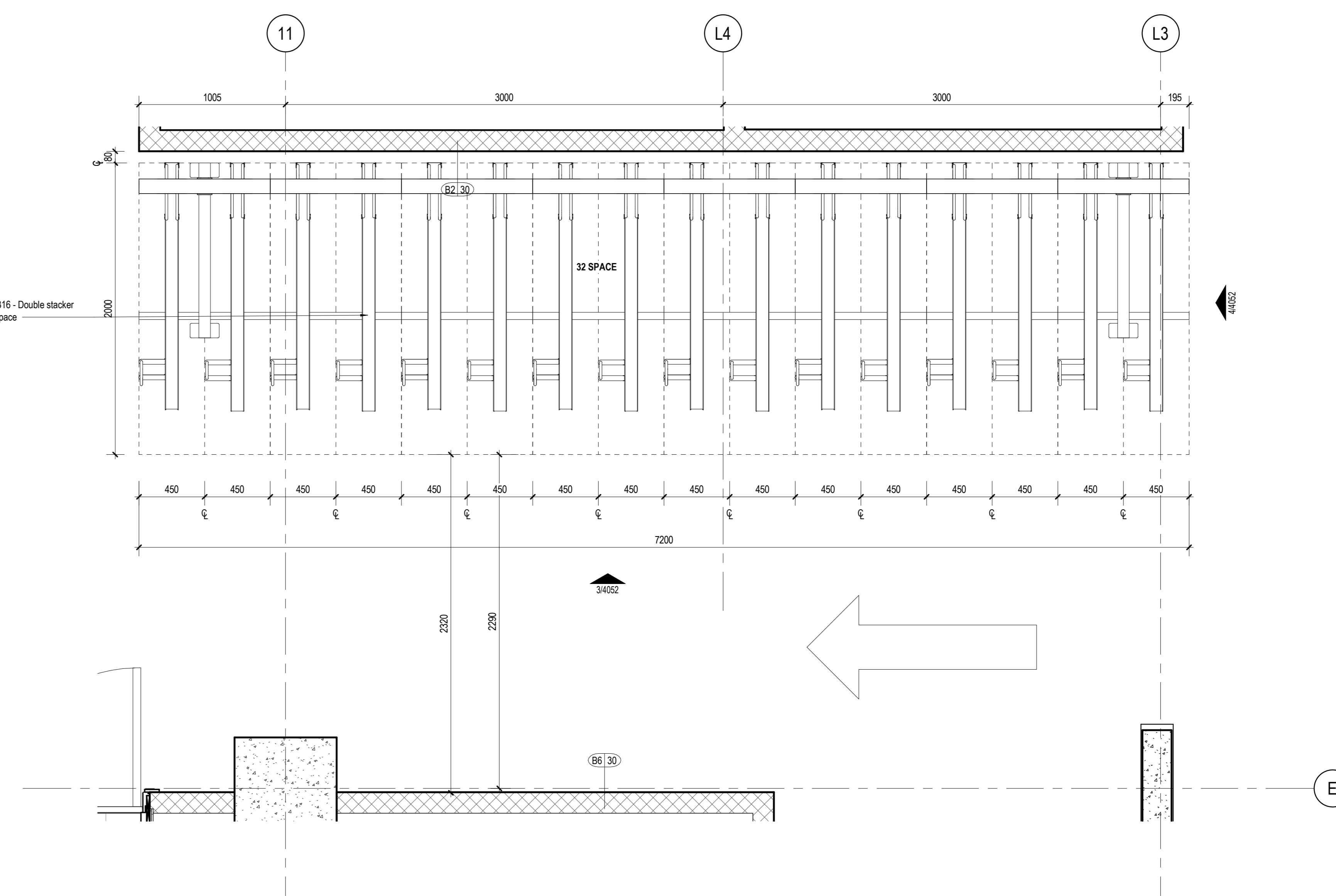
1 Enlarged Plan - Cycle Parking 2 1 : 20 Referencing View: 1/ A1B1
