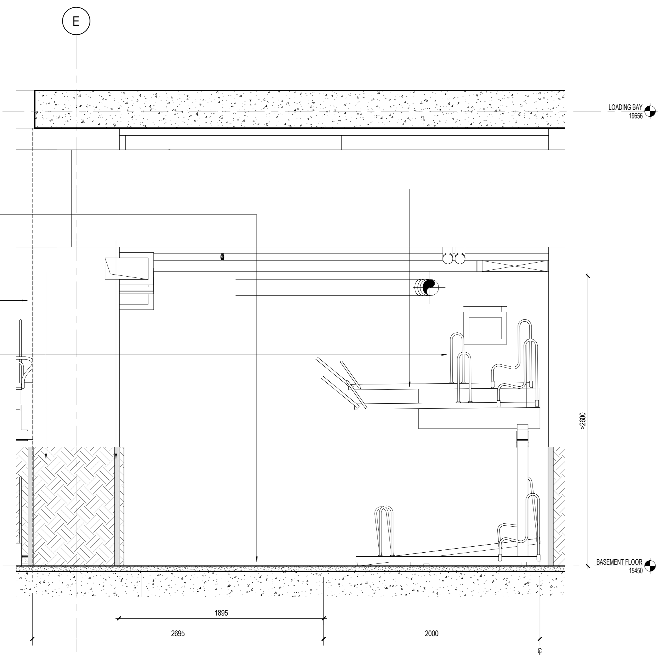
4 Enlarged Elevation 2 - Cycle Parking 2 1 : 20 Referencing View: 2/ A0
