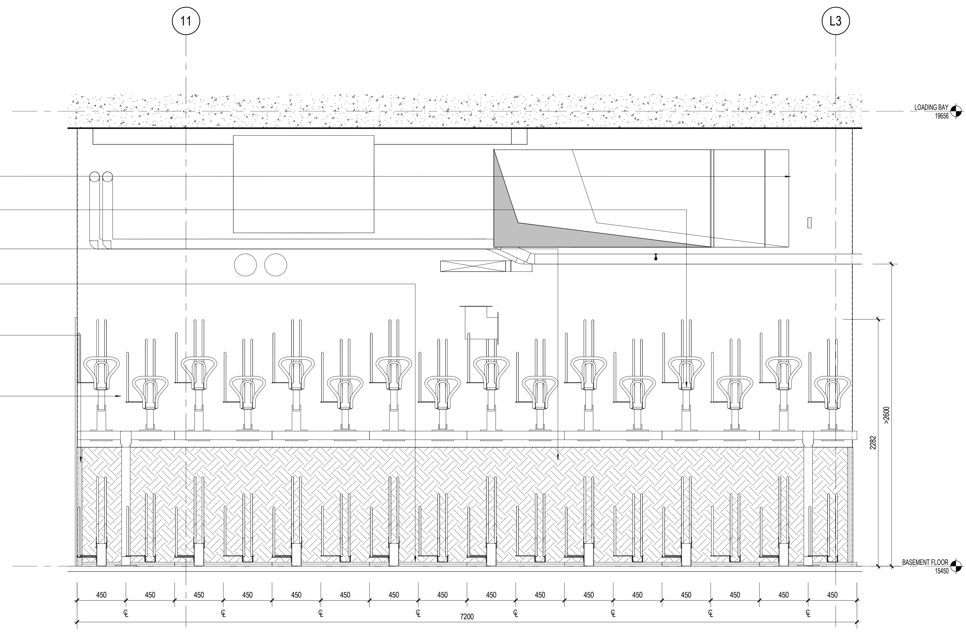
3 Enlarged Elevation 1 - Cycle Parking 2 1 : 20 Referencing View: 2/ A0
