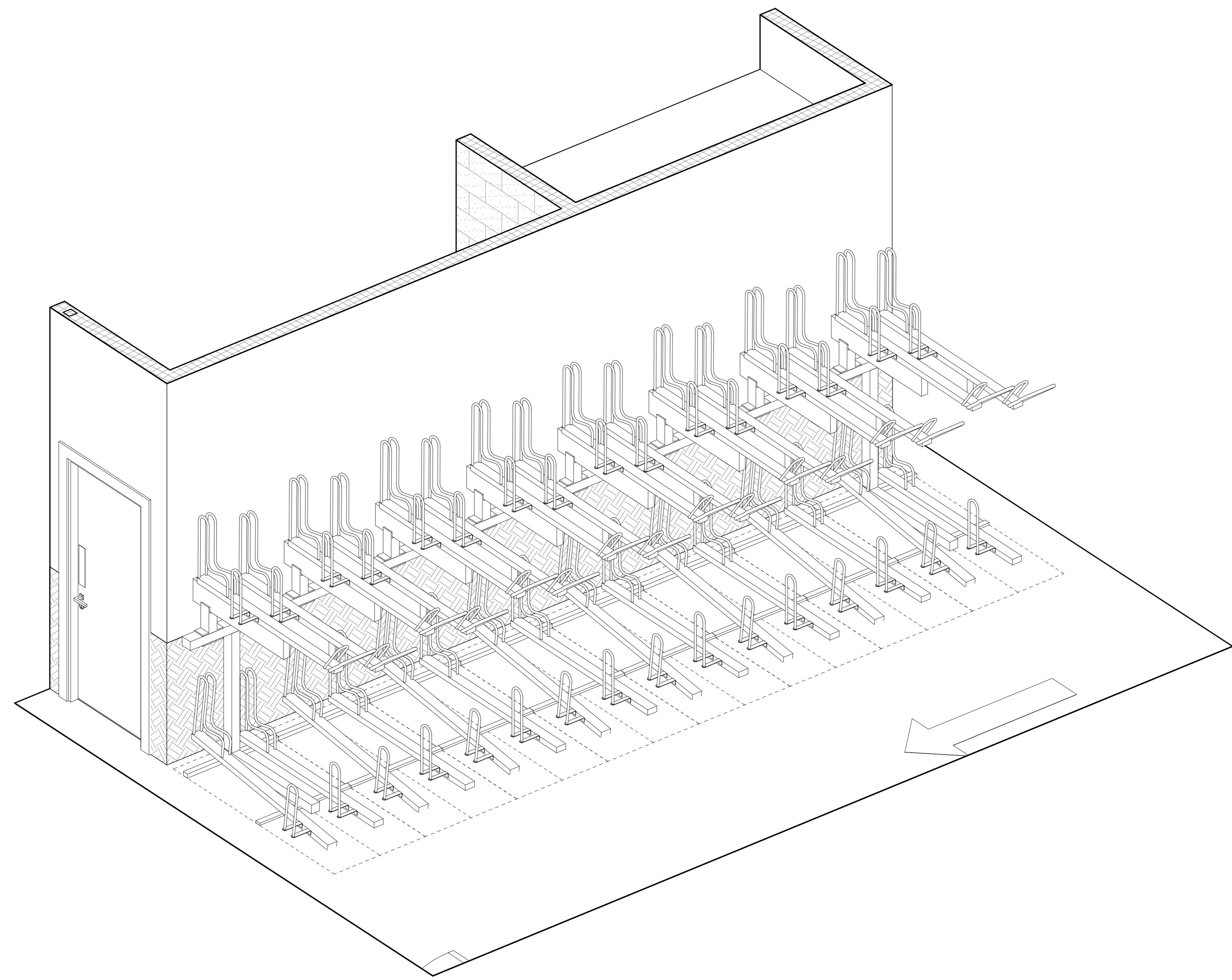
2 Cycle Parking 2 - Axo
