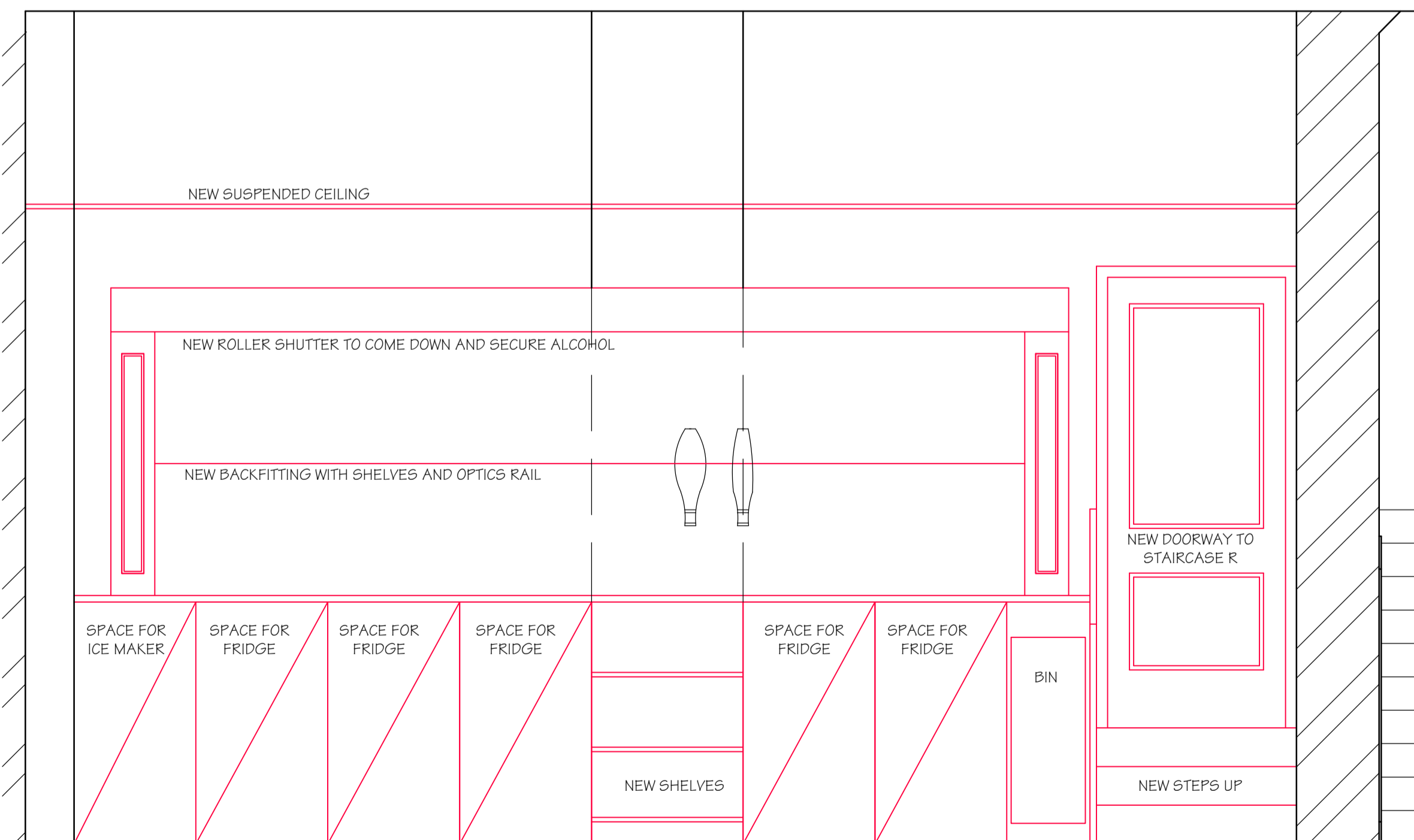
ELEVATION OF BACKFITTING (SCALE 1:20 AT A1)
