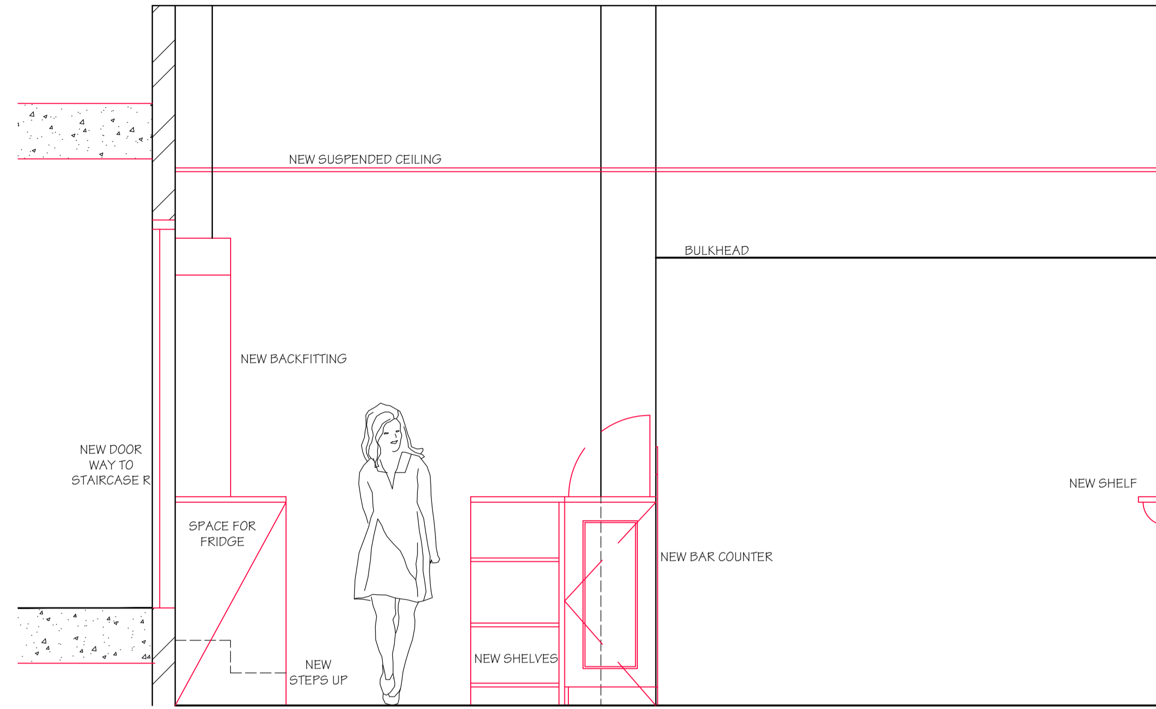
SECTION THROUGH BAR (SCALE 1:20 AT A1)
