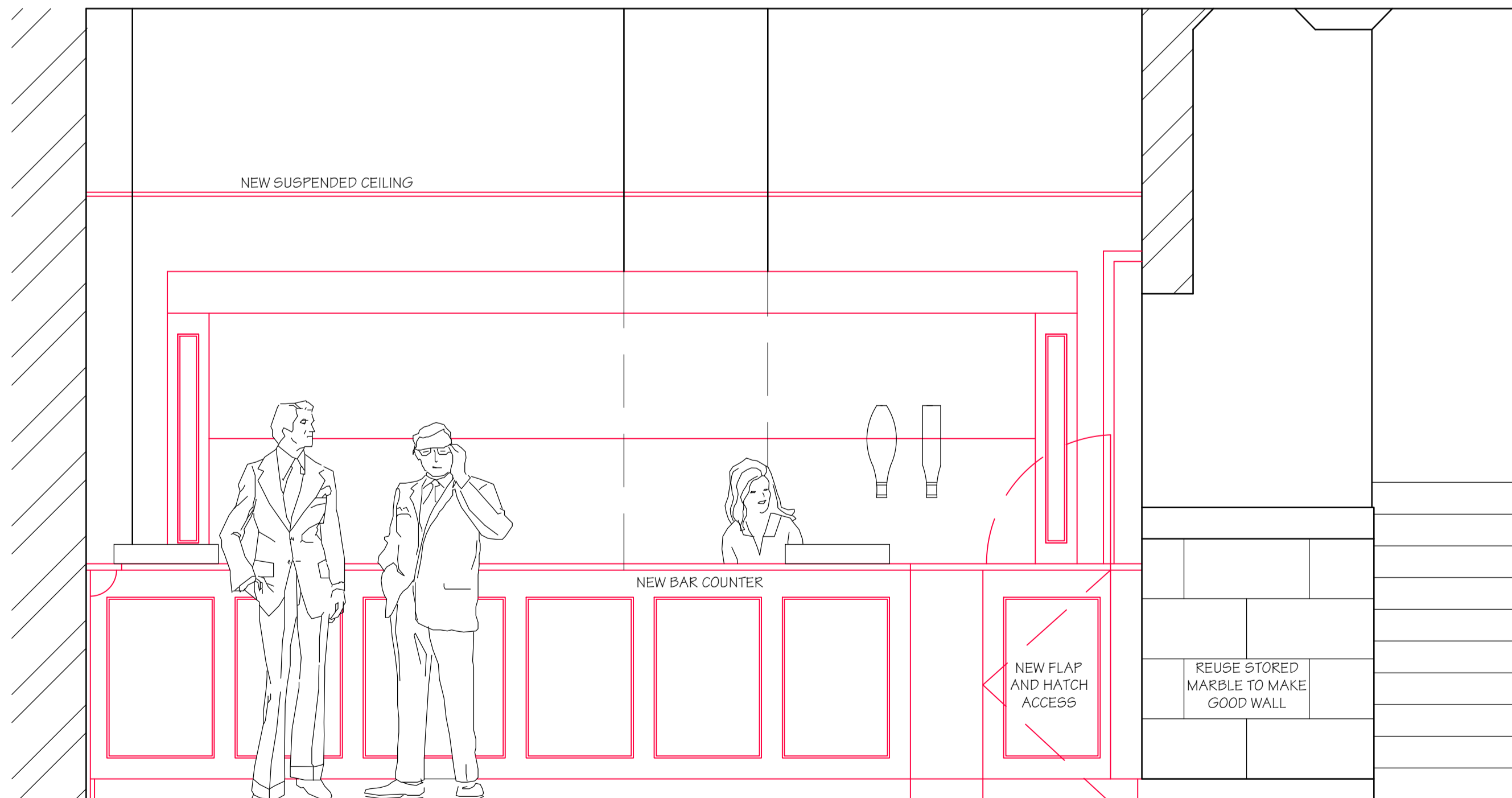
ELEVATION OF BAR (SCALE 1:20 AT A1)
