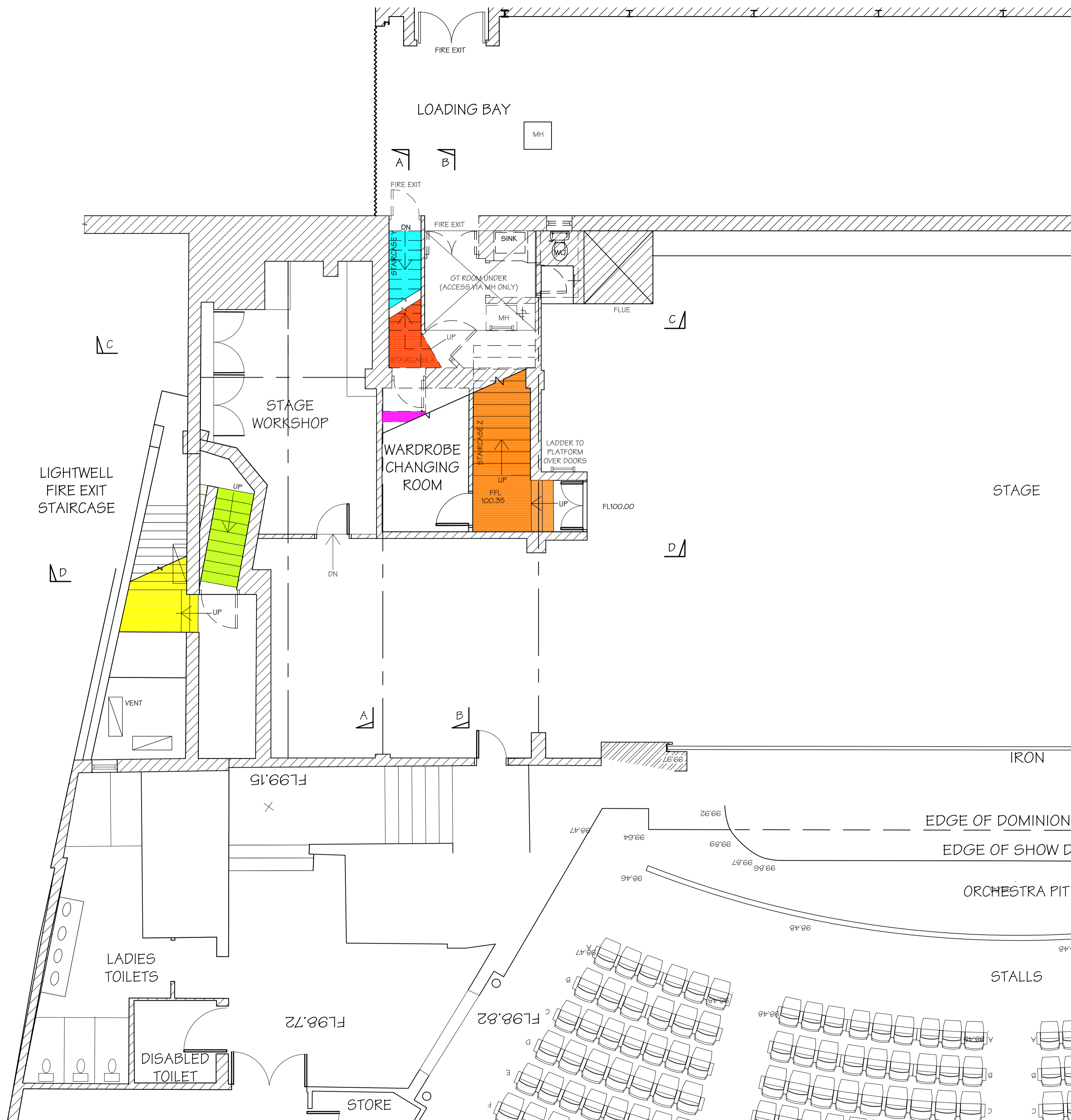
STAGE/STALLS LOWER PLAN (SCALE 1:50 AT A1)
