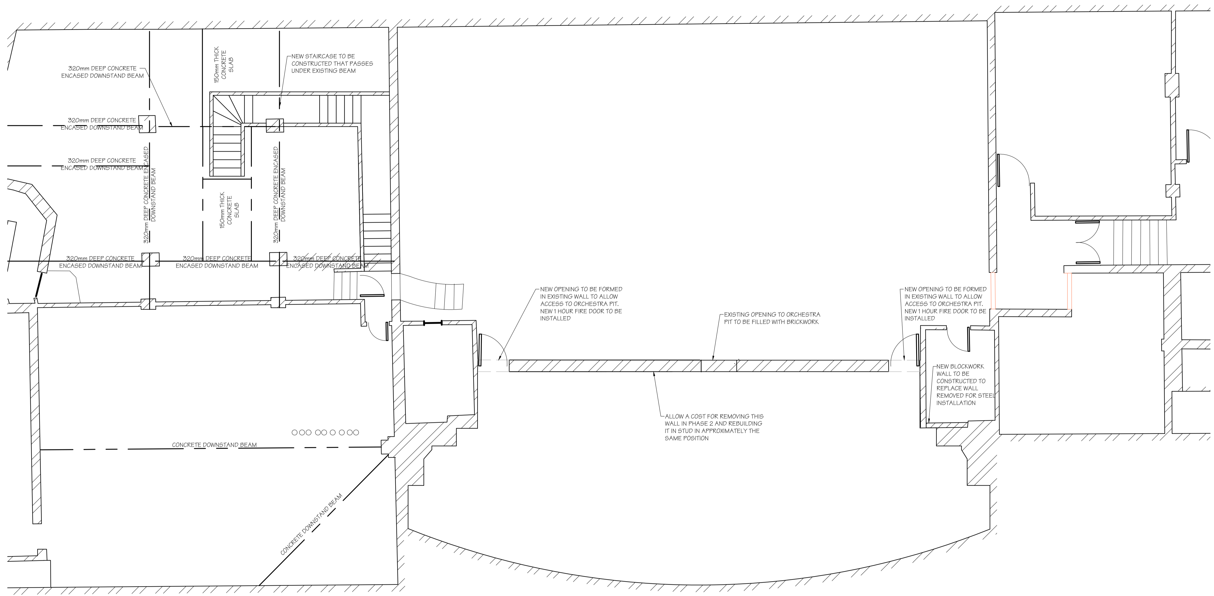
SUB STAGE PLAN SHOWING MASONRY WORK TO BE CARRIED OUT (SCALE 1:50 AT A1)
