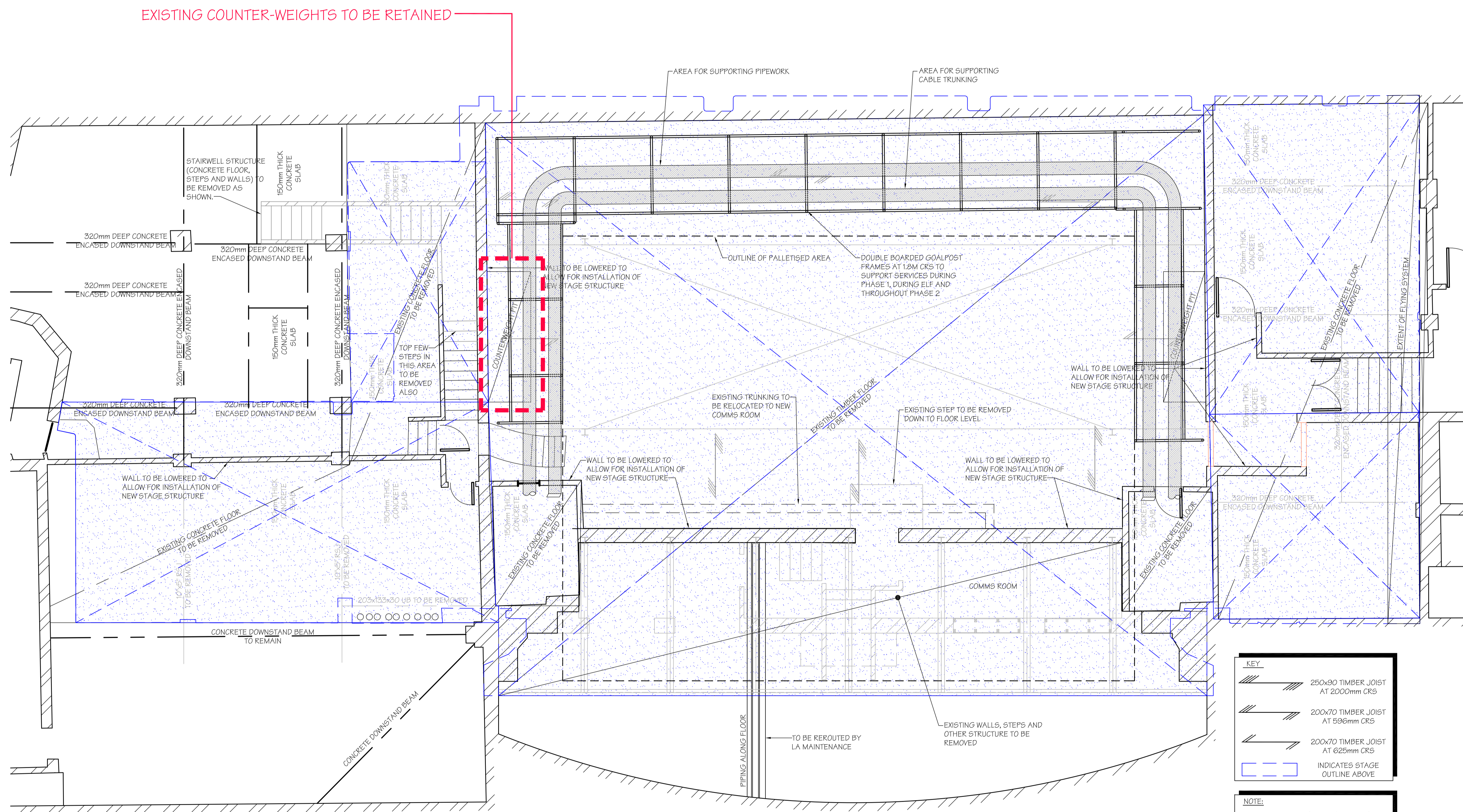
SUB STAGE PLAN SHOWING STRUCTURE TO BE REMOVED (SCALE 1:50 AT A1)
