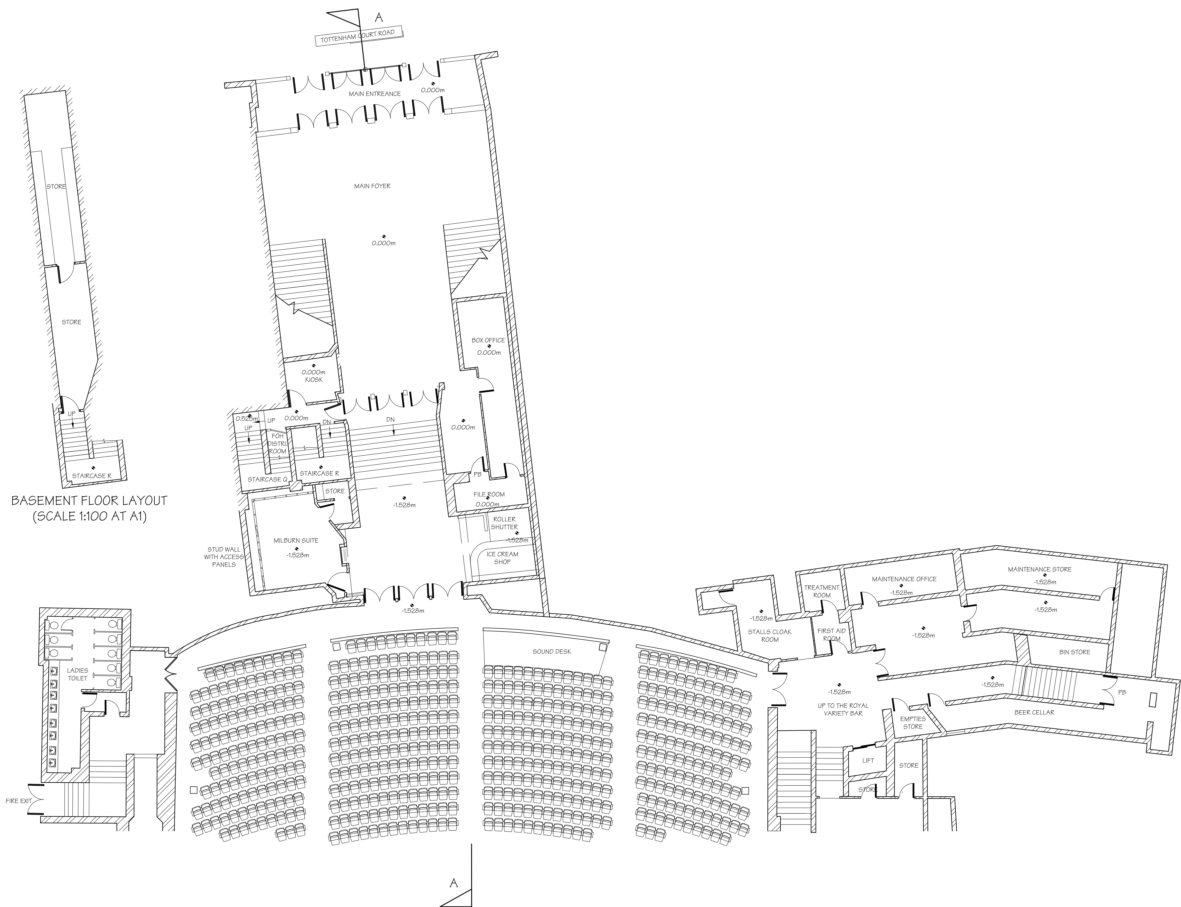
EXISTING PLAN AT GROUND FLOOR LEVEL (SCALE 1:100 AT A1)
