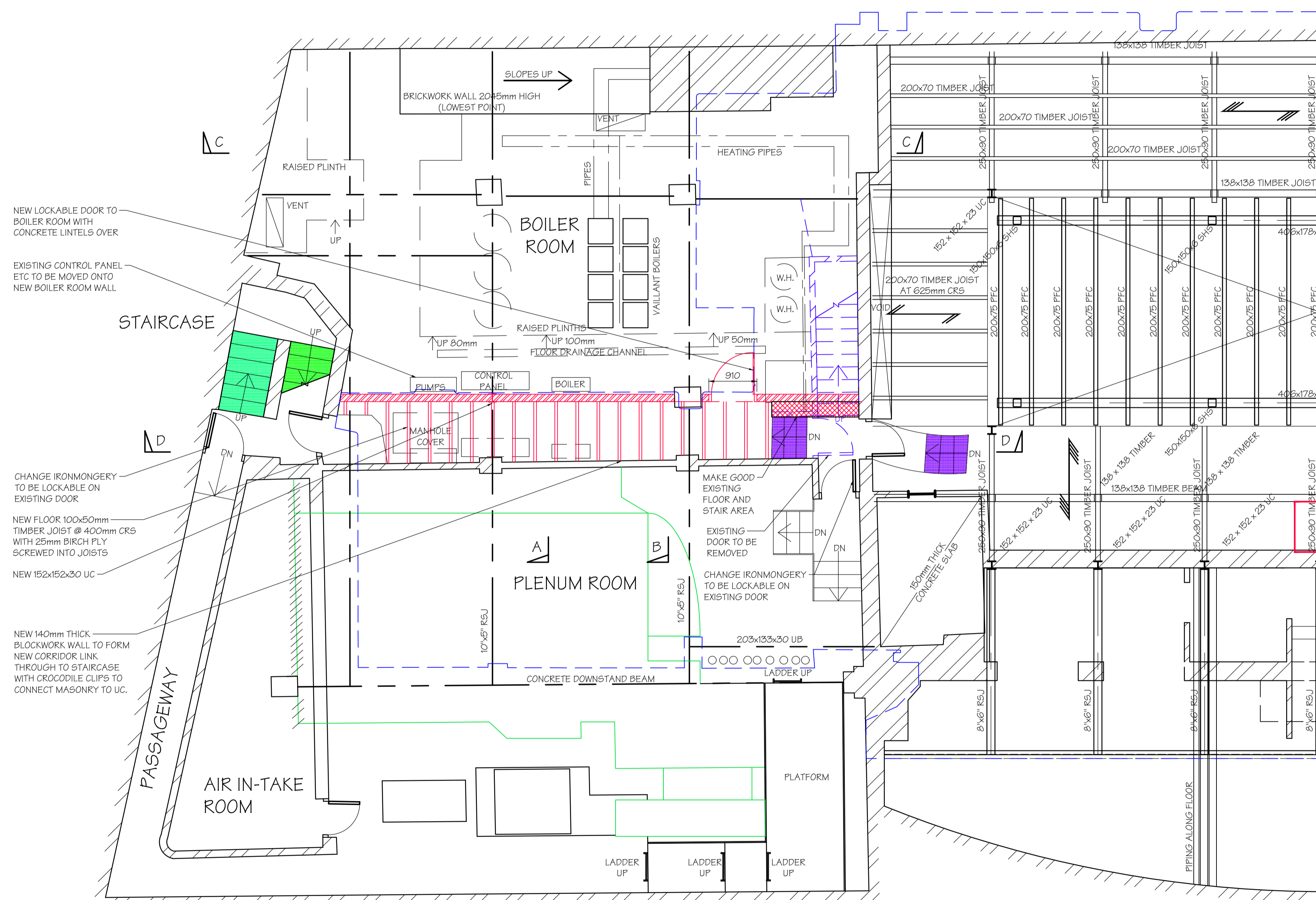
SUB STAGE LOWER PLAN SHOWING STRUCTURE ABOVE (SCALE 1:50 AT A1)
