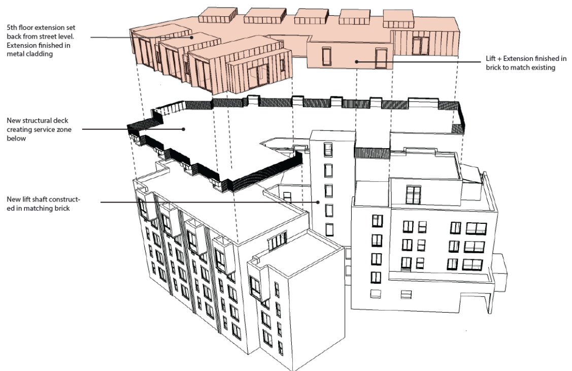
Figure 1.1: Proposed extension in relation to the existing development
