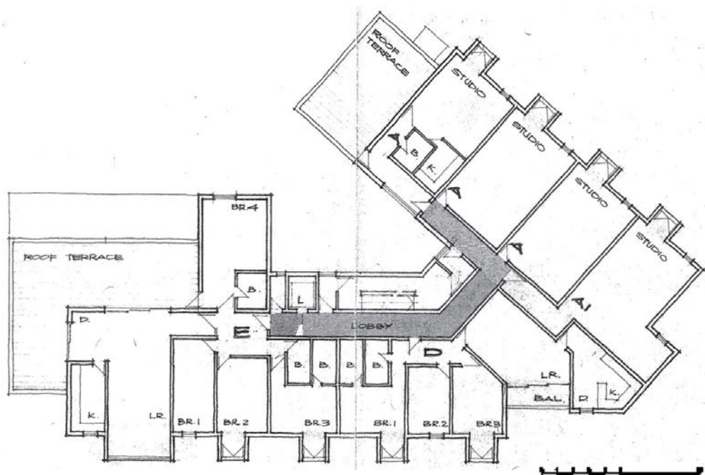
Existing Fourth Floor Plan
