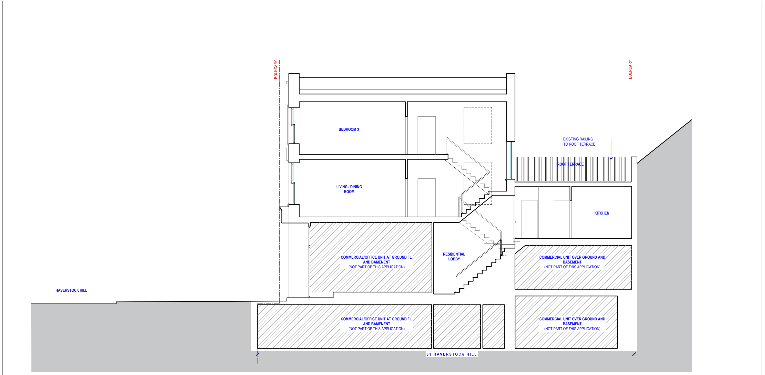
[01] EXISTING SECTION AA'
