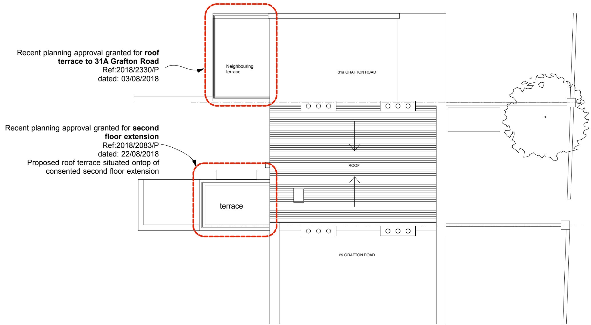
ROOF PLAN
