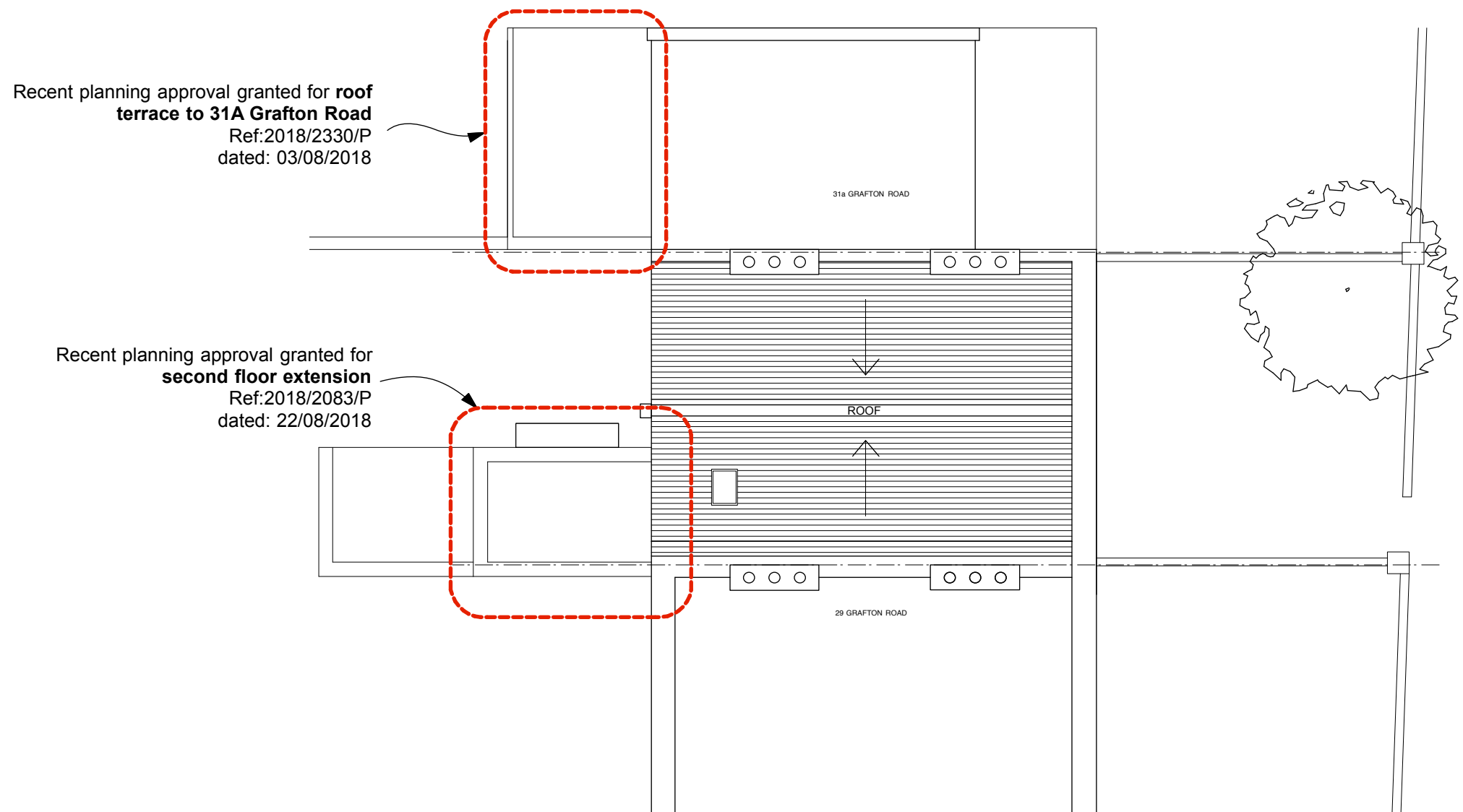
ROOF PLAN
