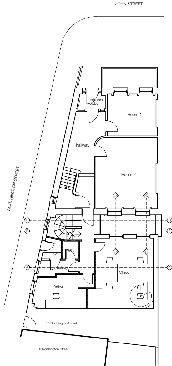
GROUND FLOOR 1:50
