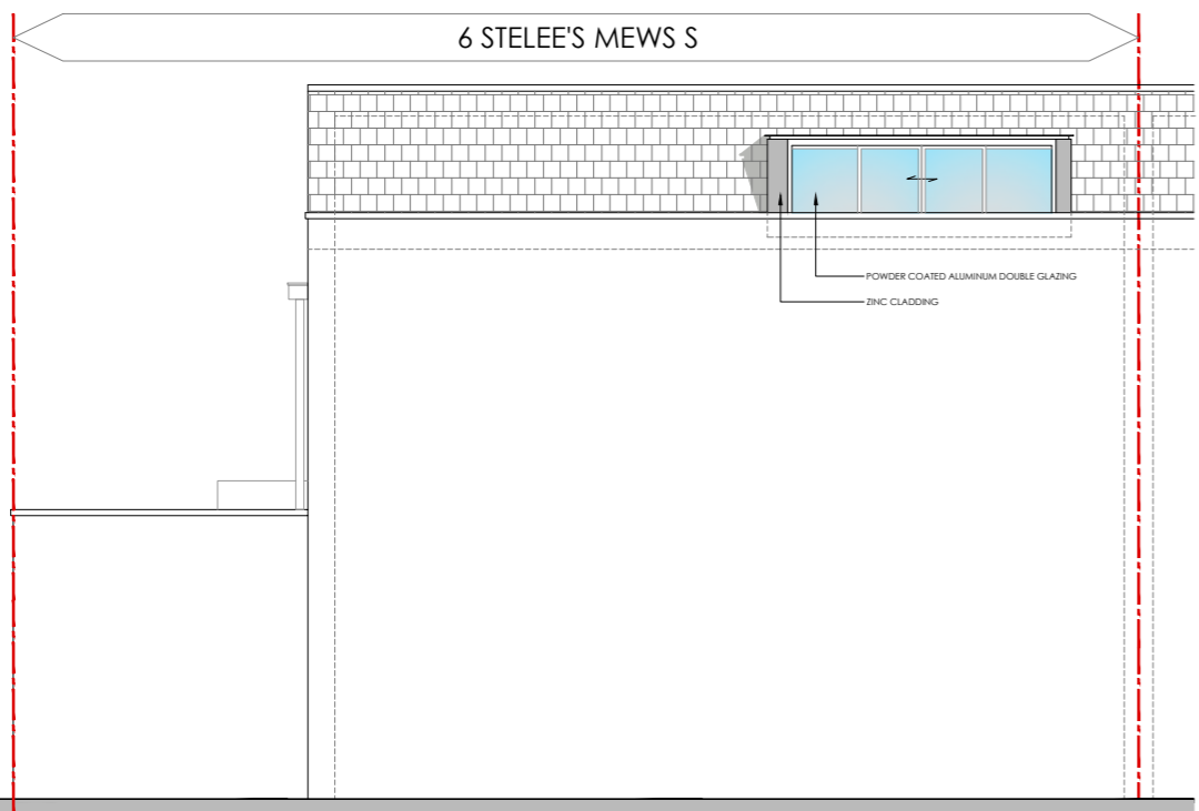
4 SOUTH EAST ELEVATION PROPOSED 1:100
