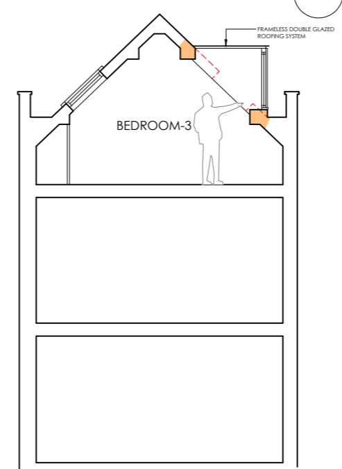
5 SECTION - A PROPOSED 1:100
