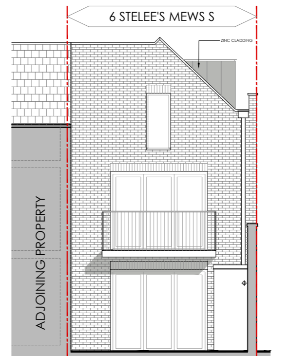
6 COURTYARD GARDEN ELEVATION PROPOSED 1:100
