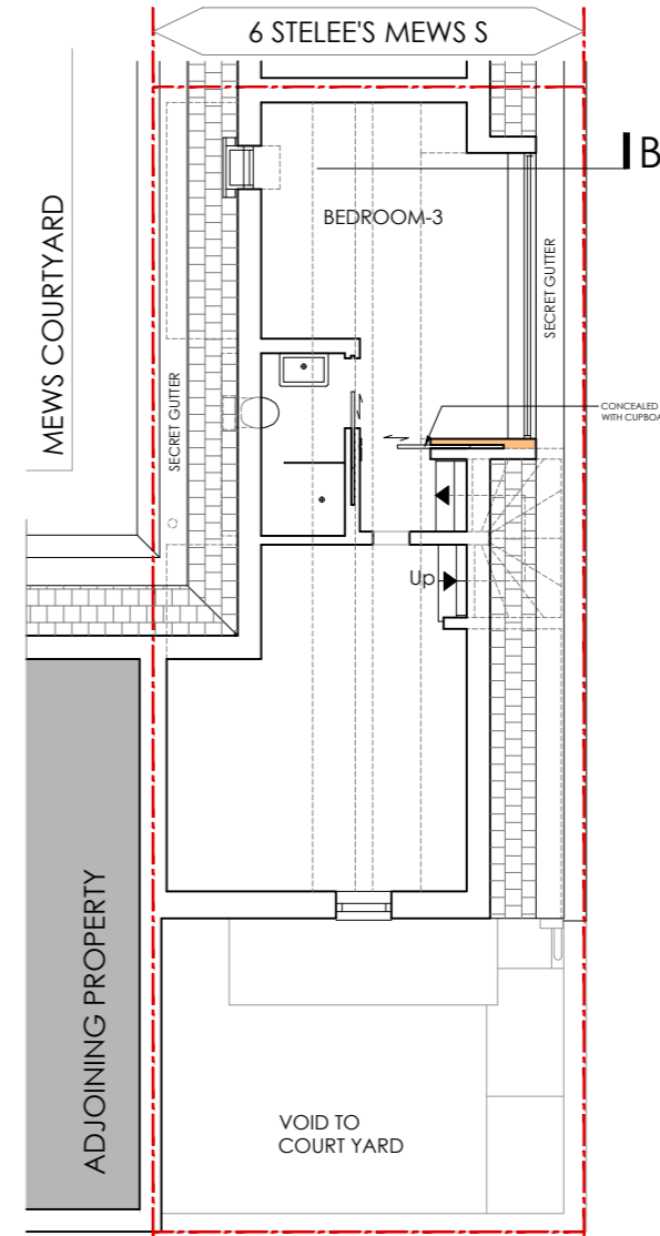
3 SECOND FLOOR PLAN PROPOSED 1:100
