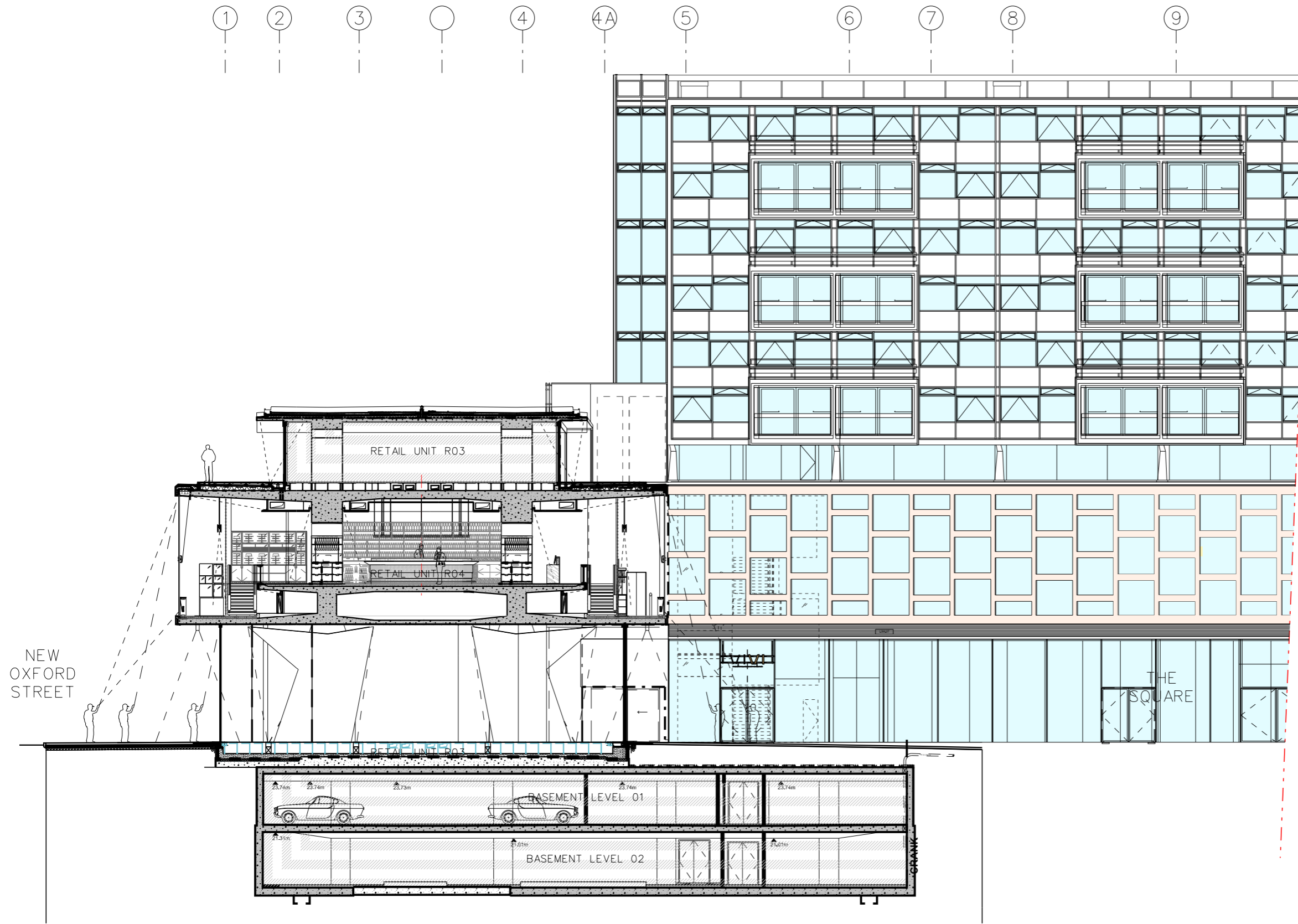
① WEST ELEVATION EXISTING 1:100
