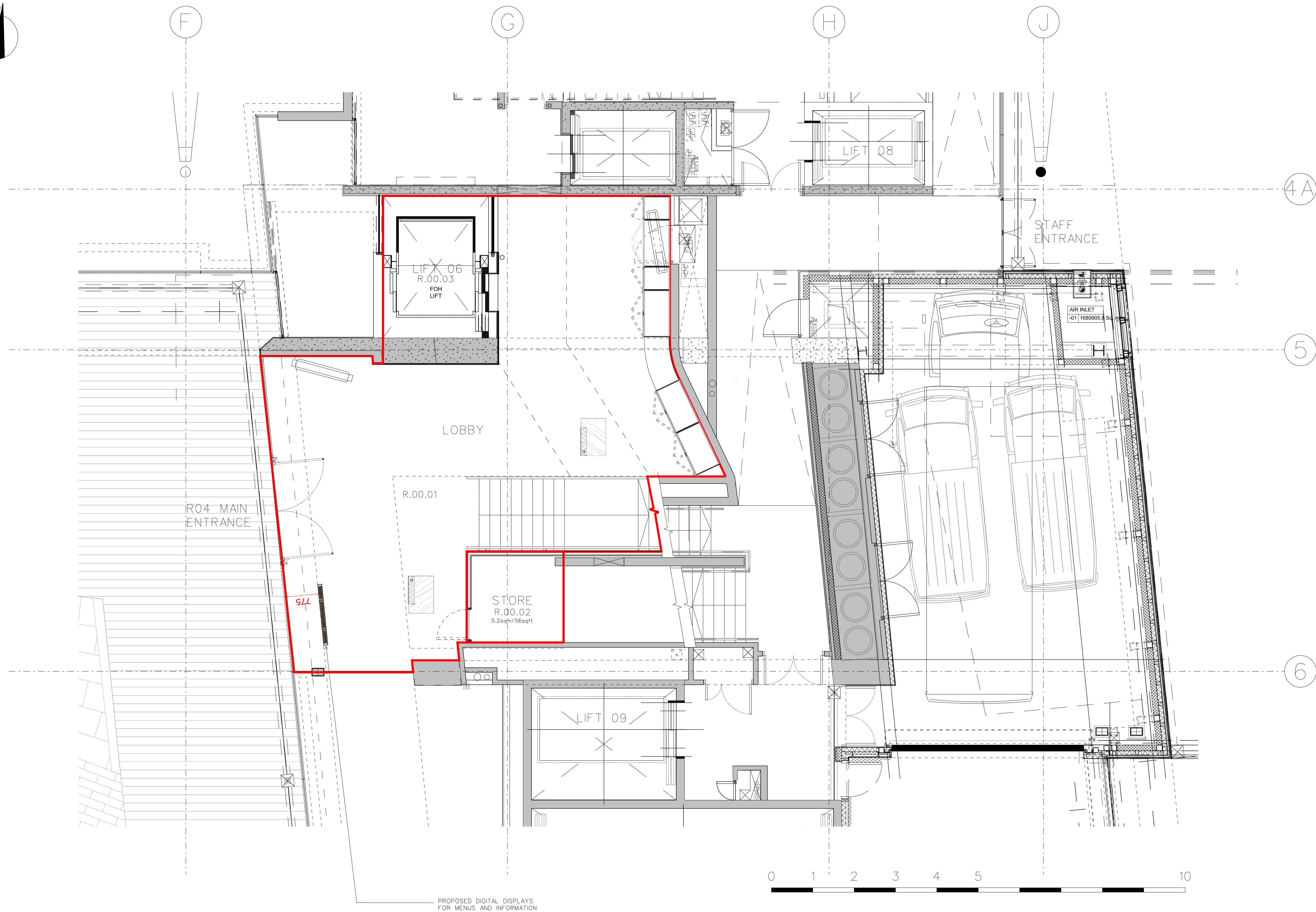
1 LEVEL 00 - PLAN PROPOSED 1:50
