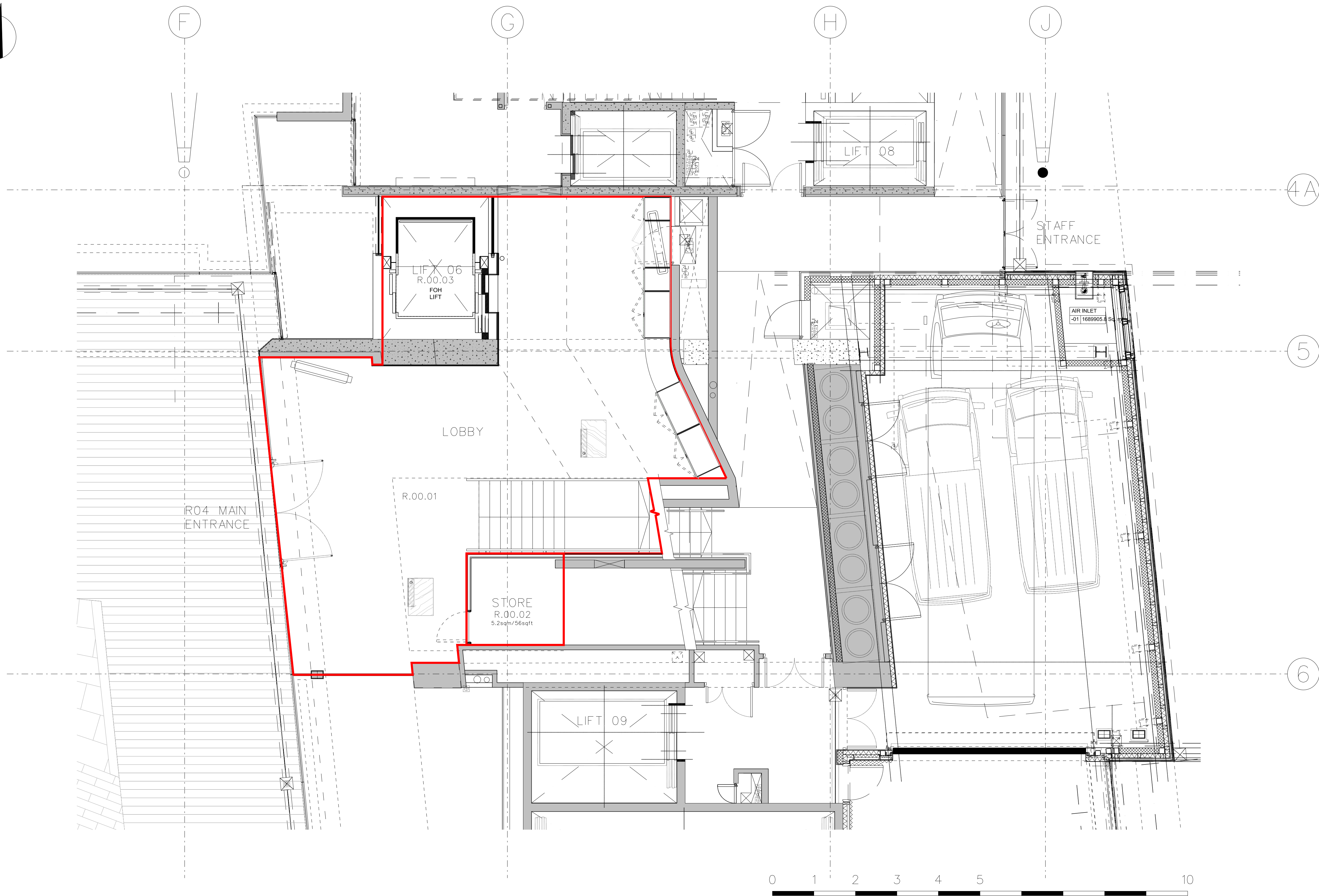
① LEVEL 00 - PLAN PROPOSED 1:50
