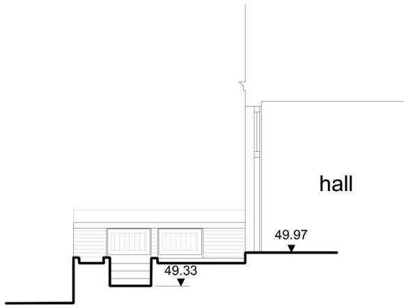
Section C-C
