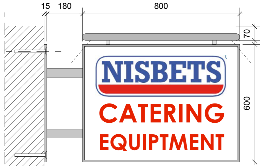
Royal College Street Blade Sign Detail
