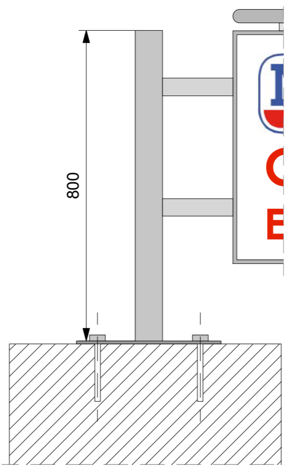
Randolf Street Brick Pier Detail
