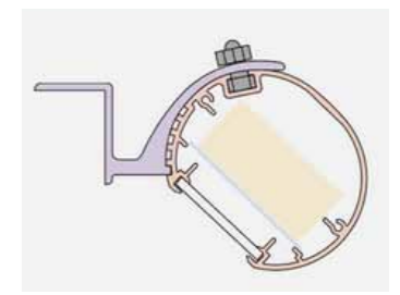
LED Downlight + Baffle
