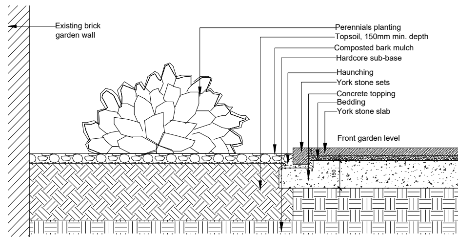
4 Detail 4: Border planting at front garden level 1:20 @ A3
