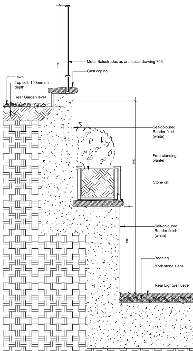
1 Detail 1: Retaining wall to rear garden level 1:20 @ A3
