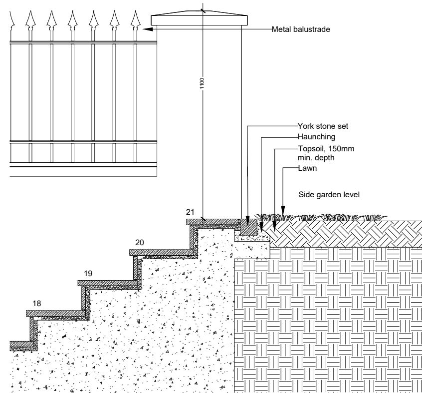
2 Detail 2: External stairs to side garden level 1:20 @ A3
