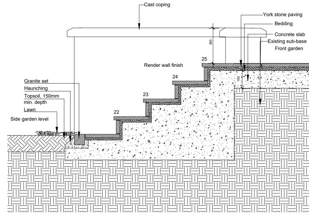
3 Detail 3: External stairs to front garden level 1:20 @ A3
