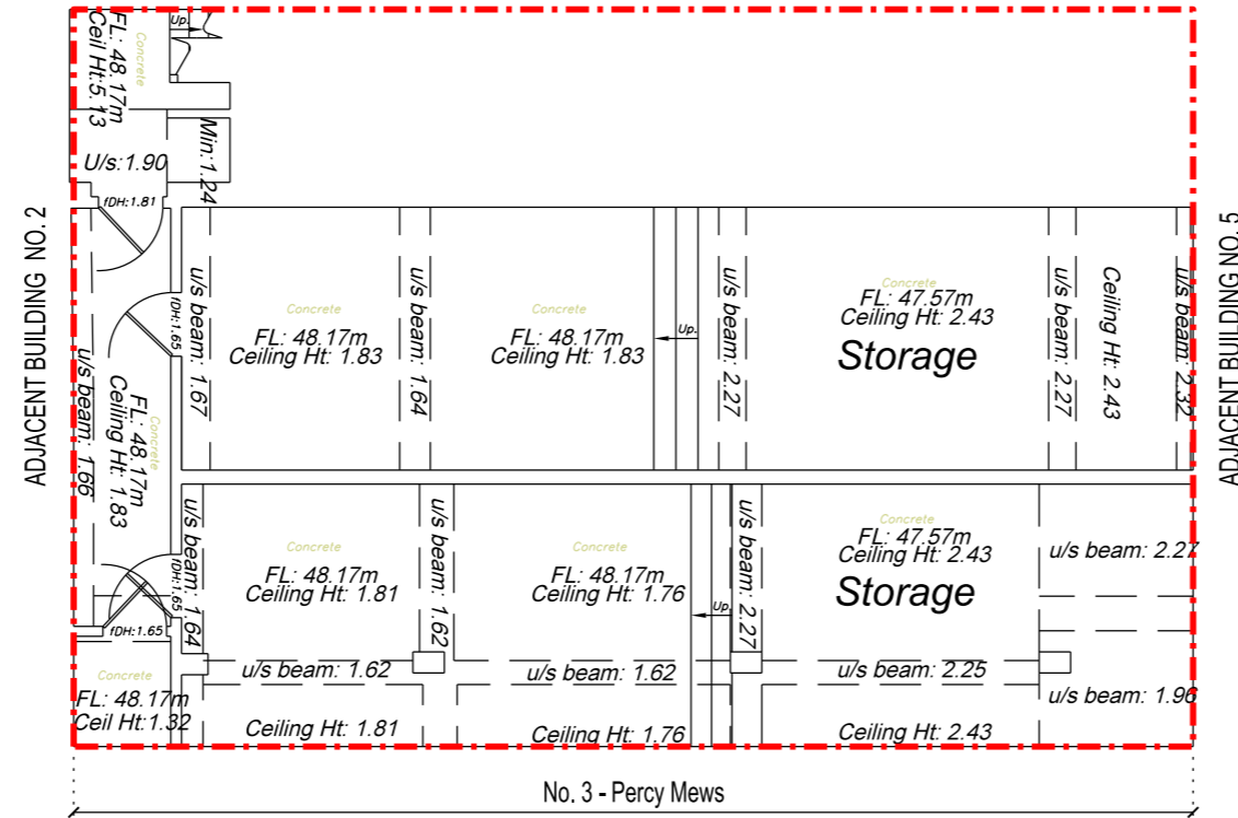
EXISTING BASEMENT PLAN
