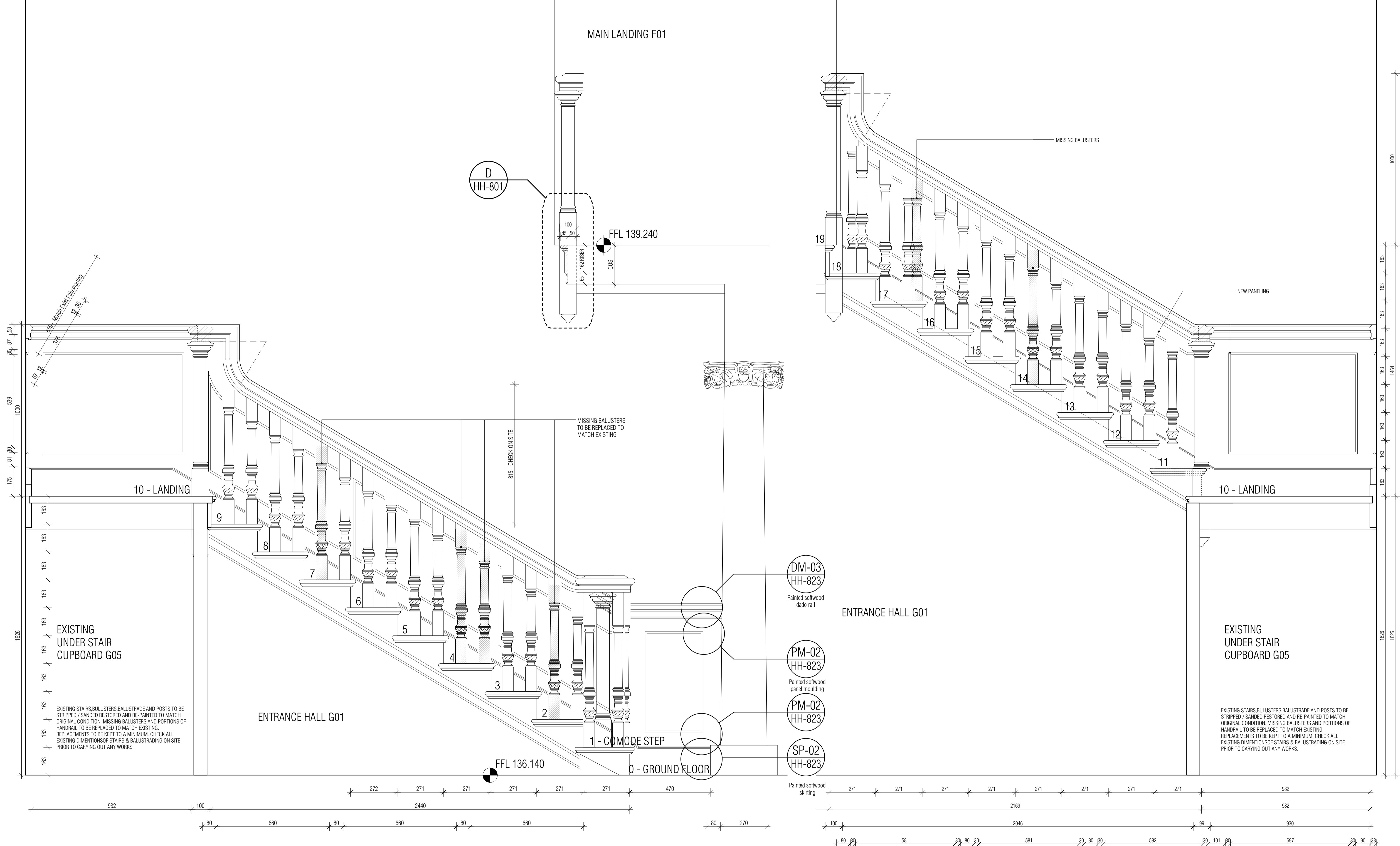
EXISTING GROUND TO FIRST FLOOR STAIRCASE & BALLUSTRADING RESTORATION ELEVATION 2/3 1:10
